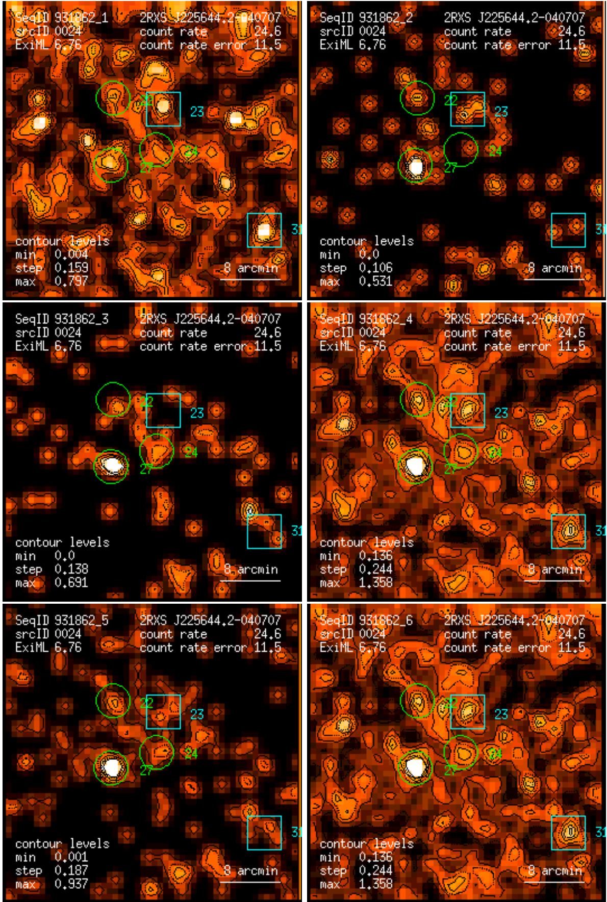
Figure 24: RASS 931862: detection 0024: band rate images, Gaussian filter: (1) PSPC channels 11 – 41, (2) 52 – 90, (3) 91 – 201, (4) 11 – 235, (5) 52 – 201, (6) 11 – 201. Broad band rates in counts/ks. Band rate contour levels in counts/ks/arcmin 2 .
