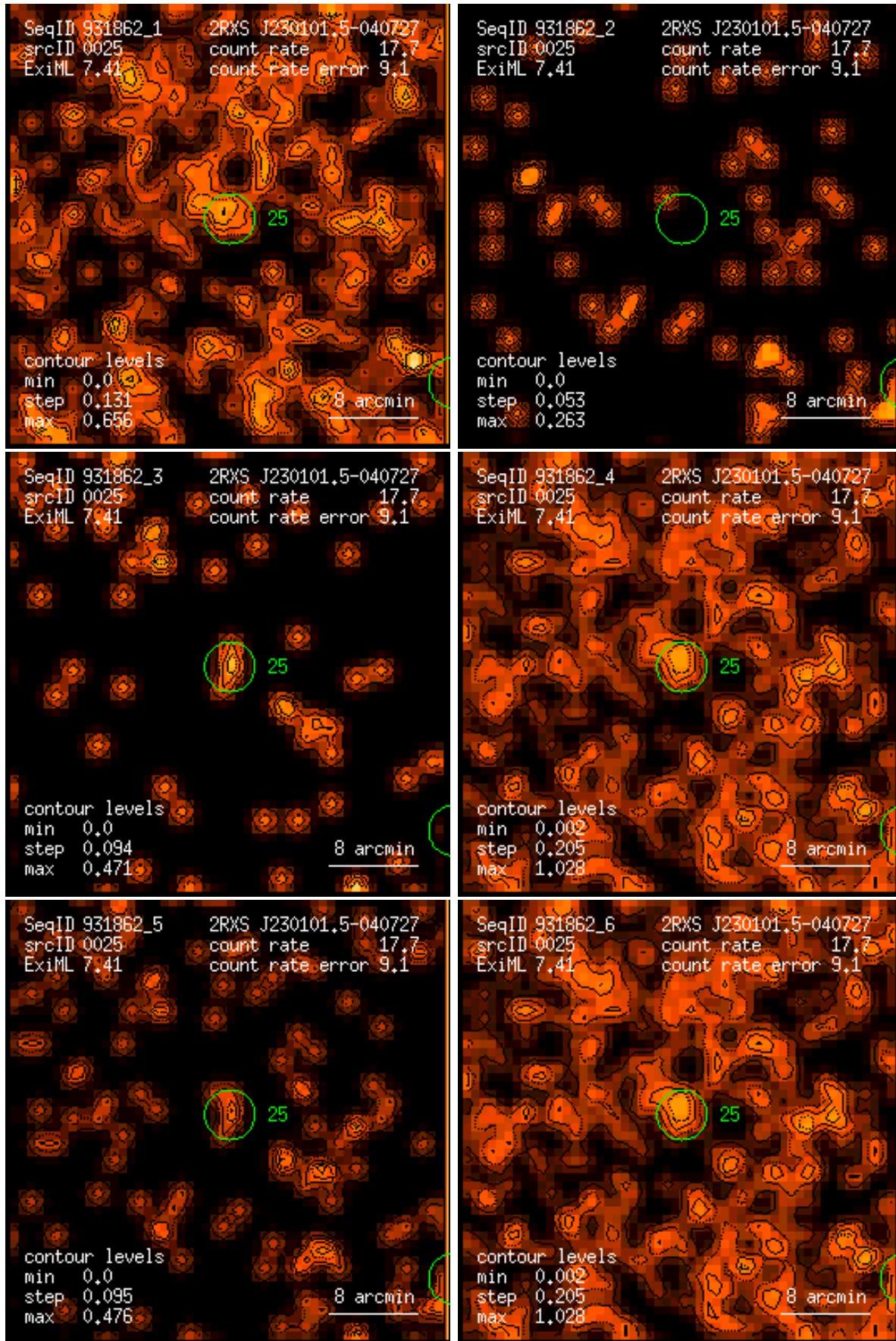
Figure 25: RASS 931862: detection 0025: band rate images, Gaussian filter: (1) PSPC channels 11 – 41, (2) 52 – 90, (3) 91 – 201, (4) 11 – 235, (5) 52 – 201, (6) 11 – 201. Broad band rates in counts/ks. Band rate contour levels in counts/ks/arcmin 2 .
