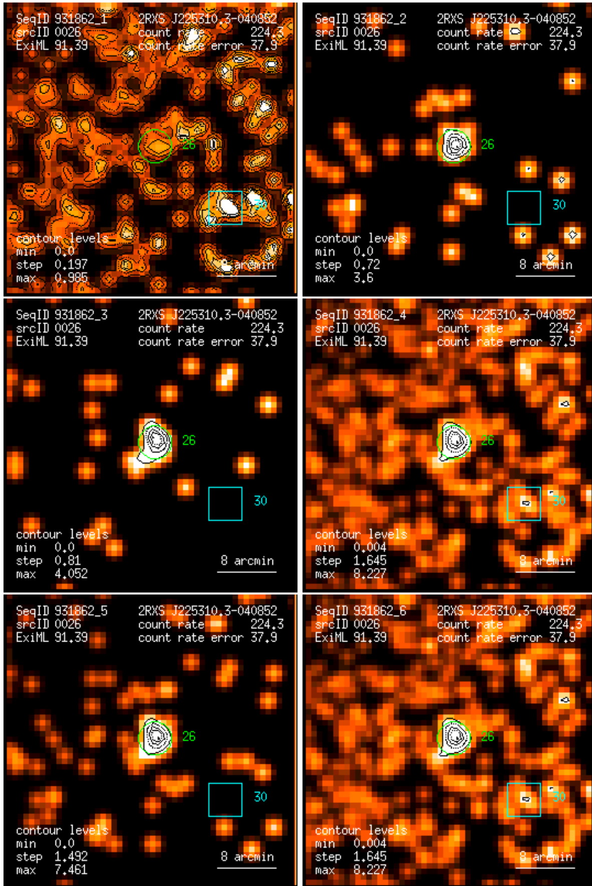
Figure 26: RASS 931862: detection 0026: band rate images, Gaussian filter: (1) PSPC channels 11 – 41, (2) 52 – 90, (3) 91 – 201, (4) 11 – 235, (5) 52 – 201, (6) 11 – 201. Broad band rates in counts/ks. Band rate contour levels in counts/ks/arcmin 2 .
