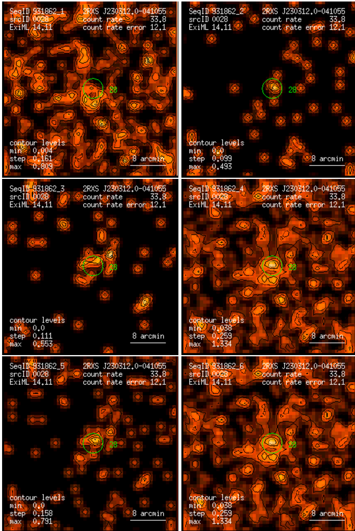
Figure 28: RASS 931862: detection 0028: band rate images, Gaussian filter: (1) PSPC channels 11 – 41, (2) 52 – 90, (3) 91 – 201, (4) 11 – 235, (5) 52 – 201, (6) 11 – 201. Broad band rates in counts/ks. Band rate contour levels in counts/ks/arcmin 2 .
