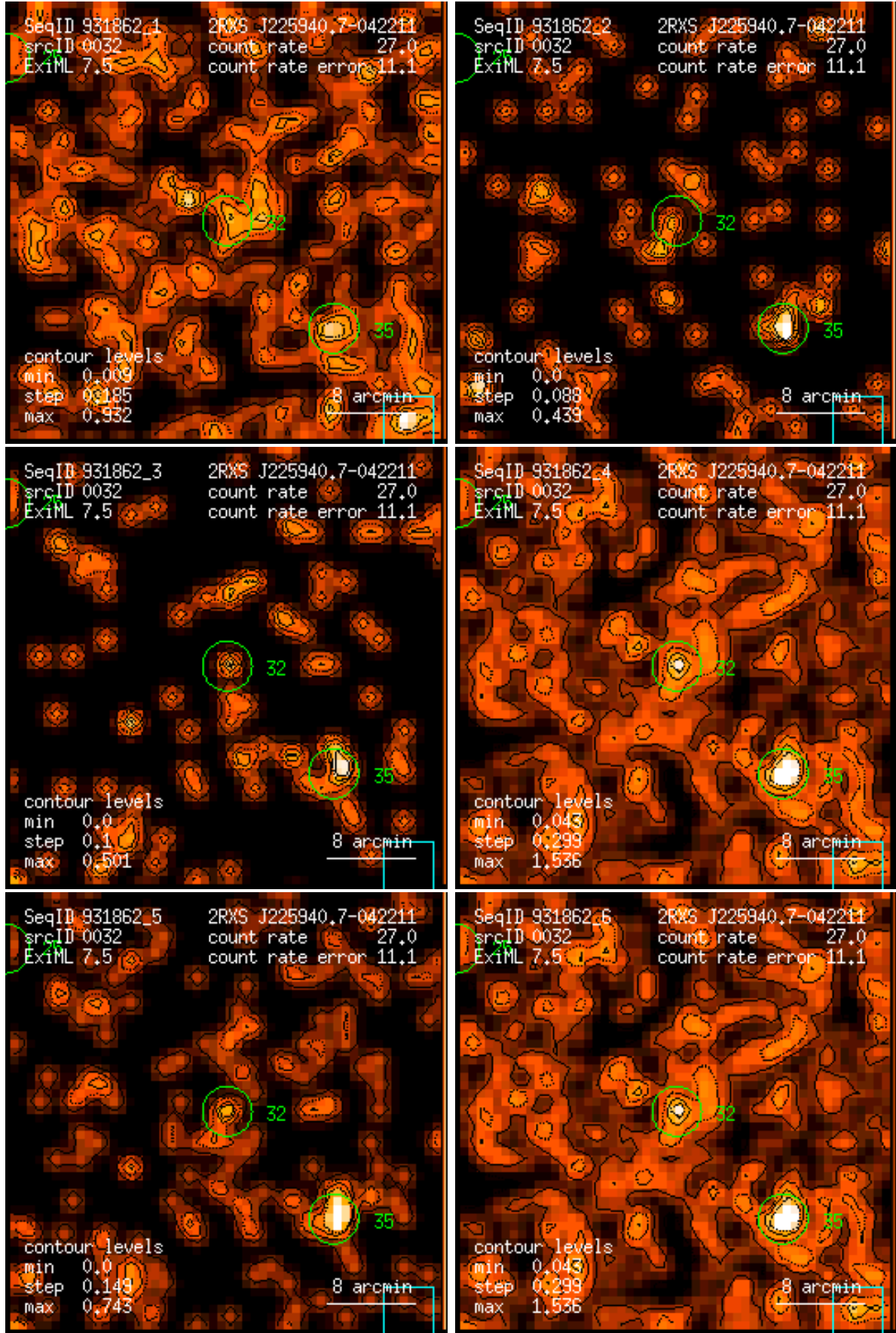
Figure 32: RASS 931862: detection 0032: band rate images, Gaussian filter: (1) PSPC channels 11 – 41, (2) 52 – 90, (3) 91 – 201, (4) 11 – 235, (5) 52 – 201, (6) 11 – 201. Broad band rates in counts/ks. Band rate contour levels in counts/ks/arcmin 2 .
