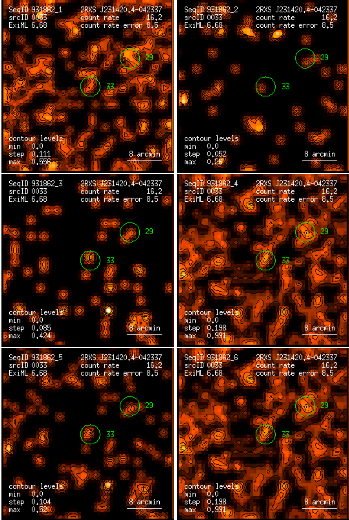
Figure 33: RASS 931862: detection 0033: band rate images, Gaussian filter: (1) PSPC channels 11 – 41, (2) 52 – 90, (3) 91 – 201, (4) 11 – 235, (5) 52 – 201, (6) 11 – 201. Broad band rates in counts/ks. Band rate contour levels in counts/ks/arcmin 2 .
