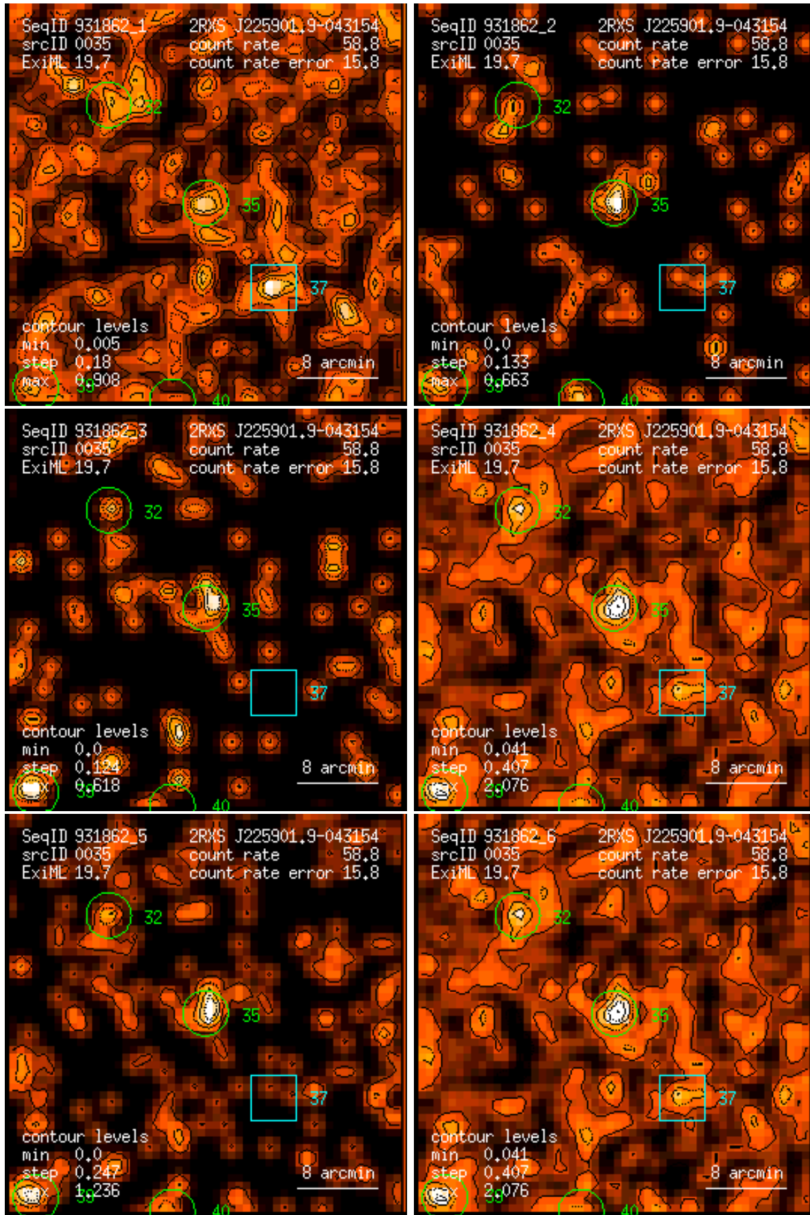
Figure 35: RASS 931862: detection 0035: band rate images, Gaussian filter: (1) PSPC channels 11 – 41, (2) 52 – 90, (3) 91 – 201, (4) 11 – 235, (5) 52 – 201, (6) 11 – 201. Broad band rates in counts/ks. Band rate contour levels in counts/ks/arcmin 2 .
