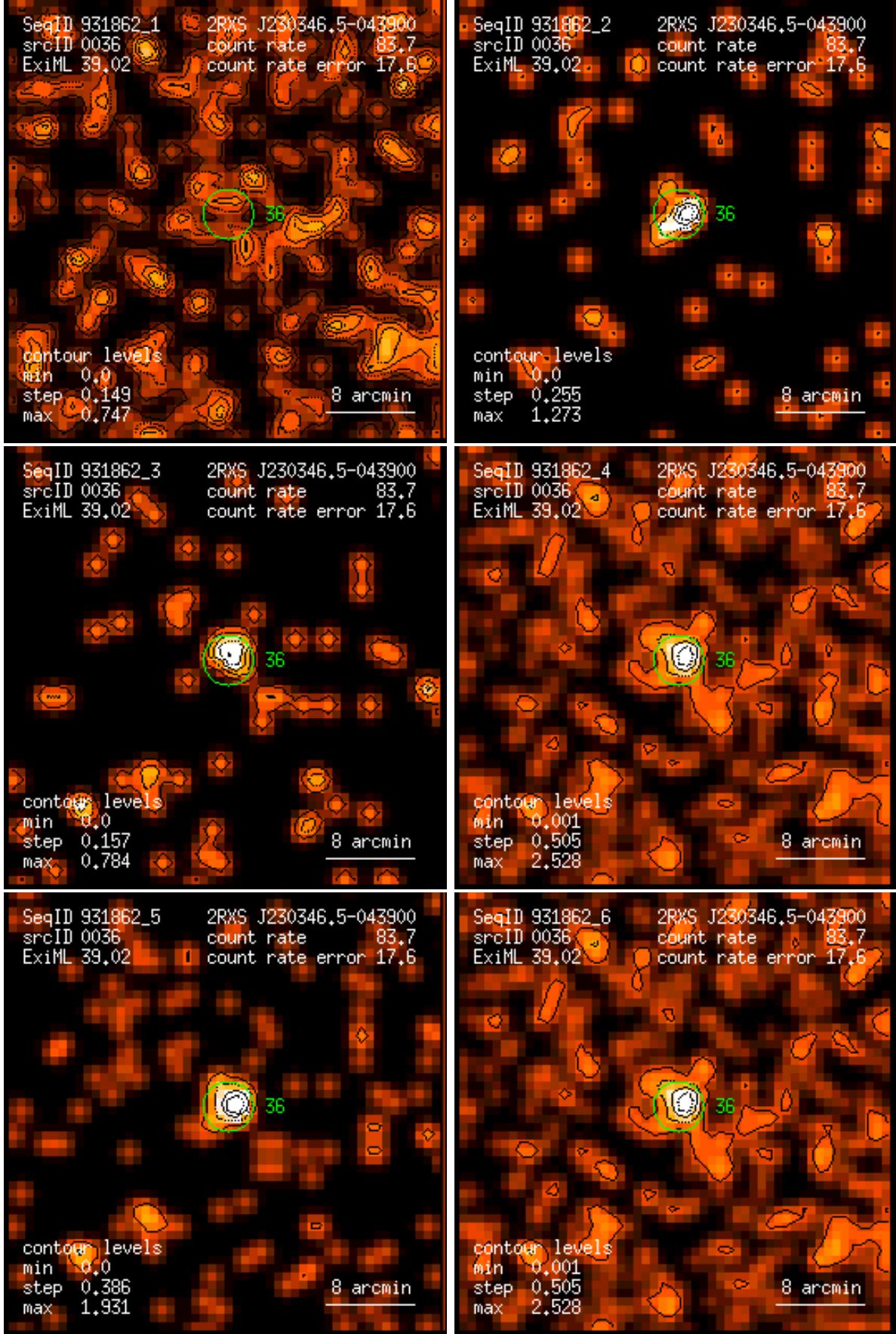
Figure 36: RASS 931862: detection 0036: band rate images, Gaussian filter: (1) PSPC channels 11 – 41, (2) 52 – 90, (3) 91 – 201, (4) 11 – 235, (5) 52 – 201, (6) 11 – 201. Broad band rates in counts/ks. Band rate contour levels in counts/ks/arcmin 2 .
