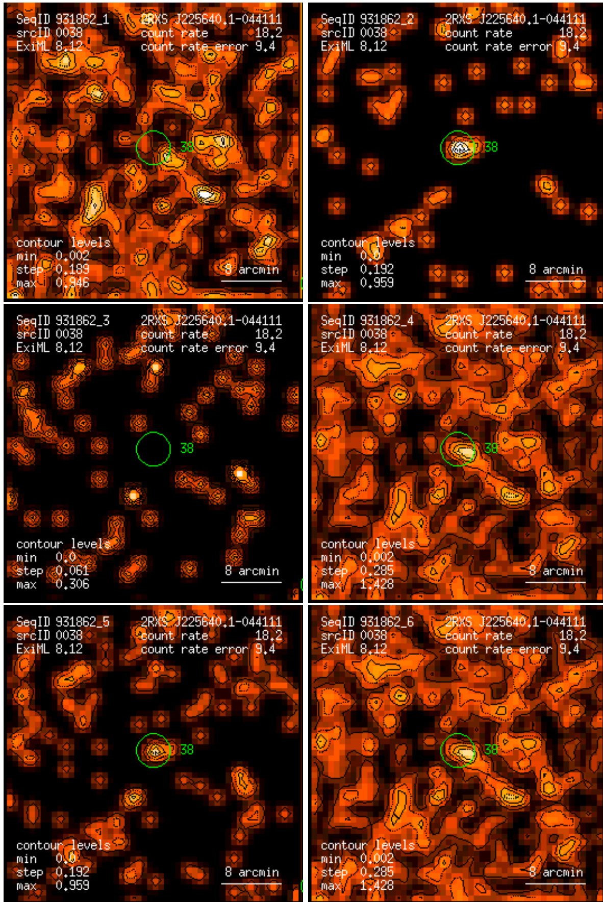
Figure 38: RASS 931862: detection 0038: band rate images, Gaussian filter: (1) PSPC channels 11 – 41, (2) 52 – 90, (3) 91 – 201, (4) 11 – 235, (5) 52 – 201, (6) 11 – 201. Broad band rates in counts/ks. Band rate contour levels in counts/ks/arcmin 2 .
