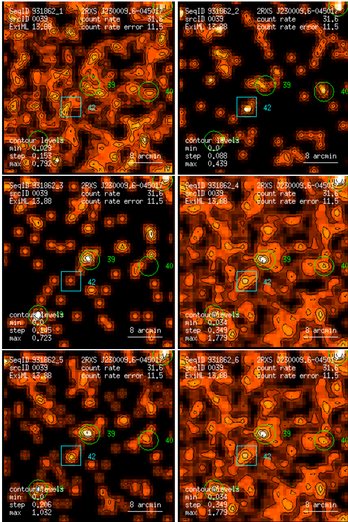
Figure 39: RASS 931862: detection 0039: band rate images, Gaussian filter: (1) PSPC channels 11 – 41, (2) 52 – 90, (3) 91 – 201, (4) 11 – 235, (5) 52 – 201, (6) 11 – 201. Broad band rates in counts/ks. Band rate contour levels in counts/ks/arcmin 2 .
