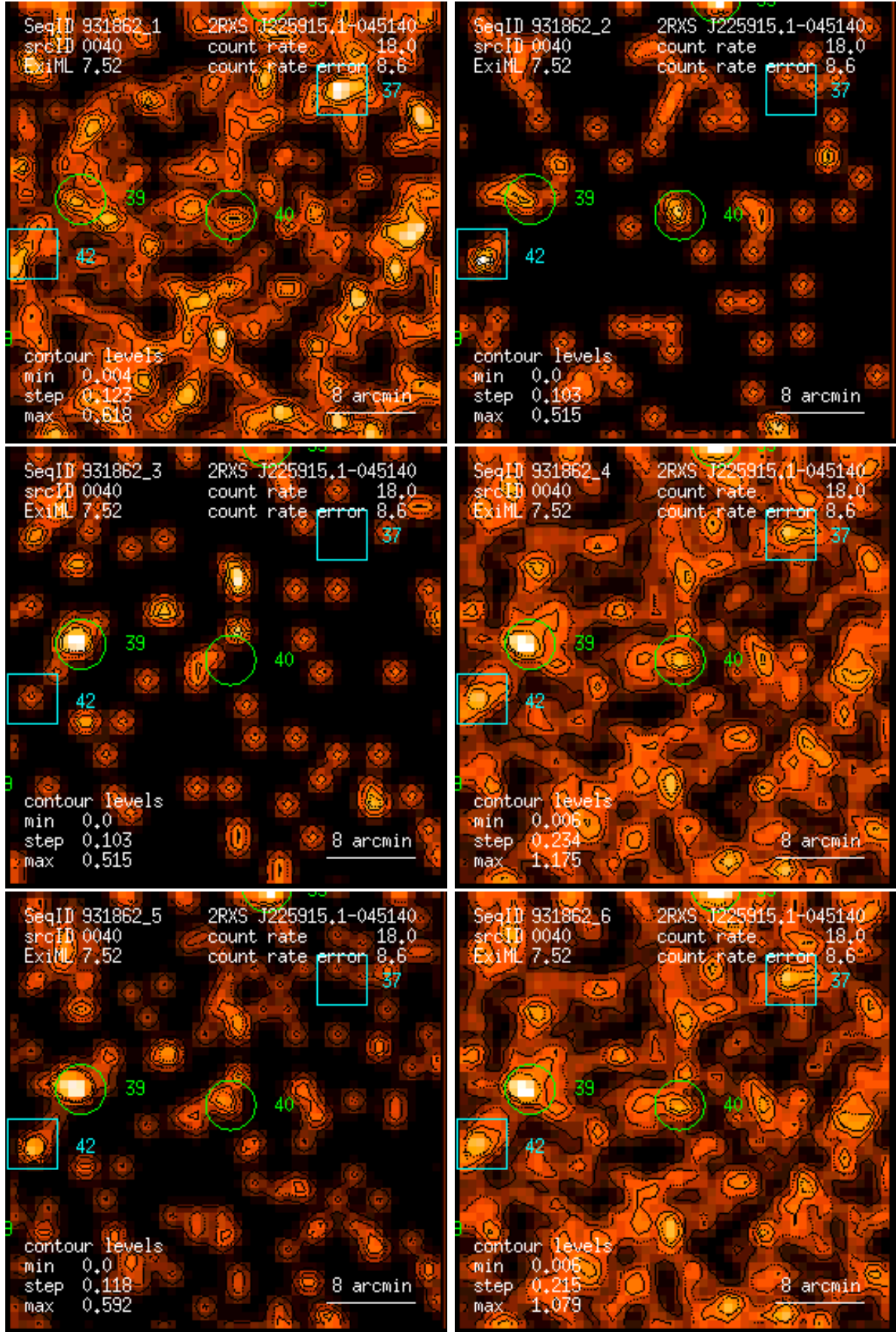
Figure 40: RASS 931862: detection 0040: band rate images, Gaussian filter: (1) PSPC channels 11 – 41, (2) 52 – 90, (3) 91 – 201, (4) 11 – 235, (5) 52 – 201, (6) 11 – 201. Broad band rates in counts/ks. Band rate contour levels in counts/ks/arcmin 2 .
