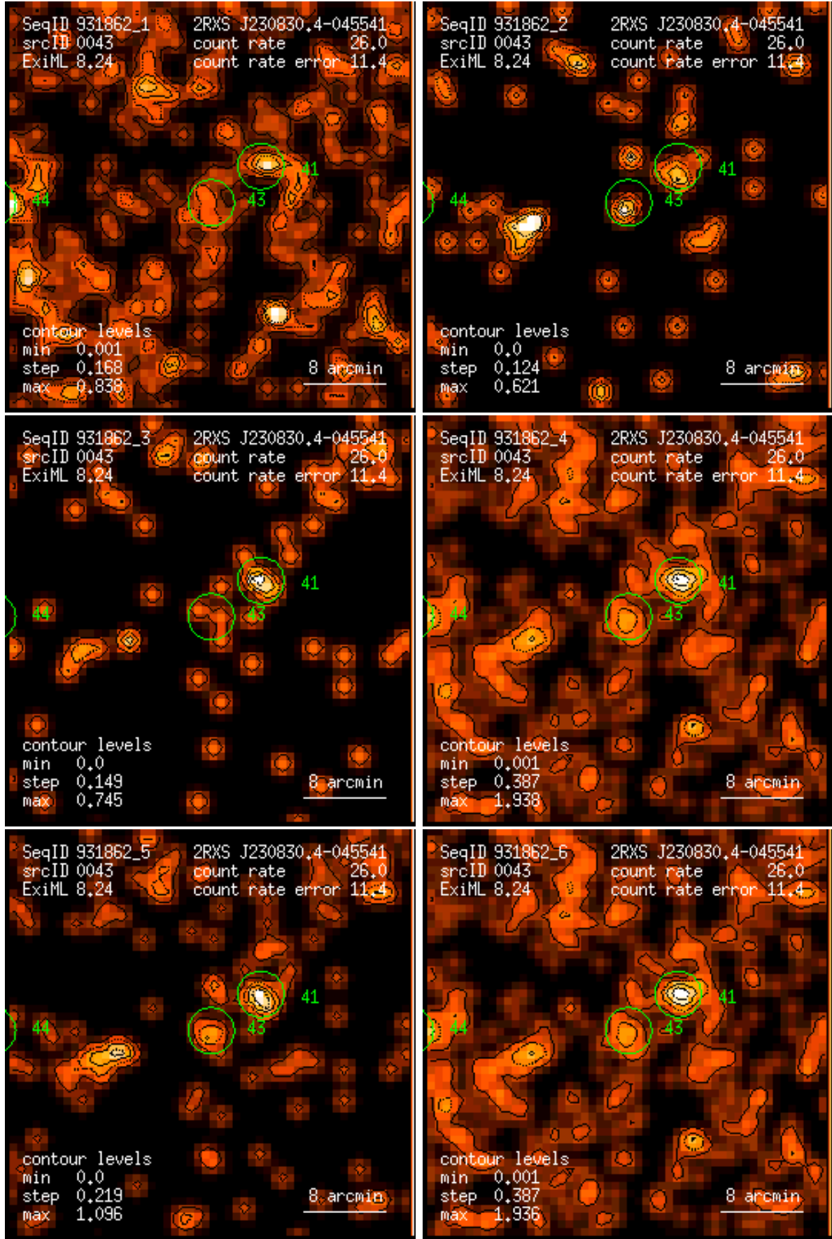
Figure 43: RASS 931862: detection 0043: band rate images, Gaussian filter: (1) PSPC channels 11 – 41, (2) 52 – 90, (3) 91 – 201, (4) 11 – 235, (5) 52 – 201, (6) 11 – 201. Broad band rates in counts/ks. Band rate contour levels in counts/ks/arcmin 2 .
