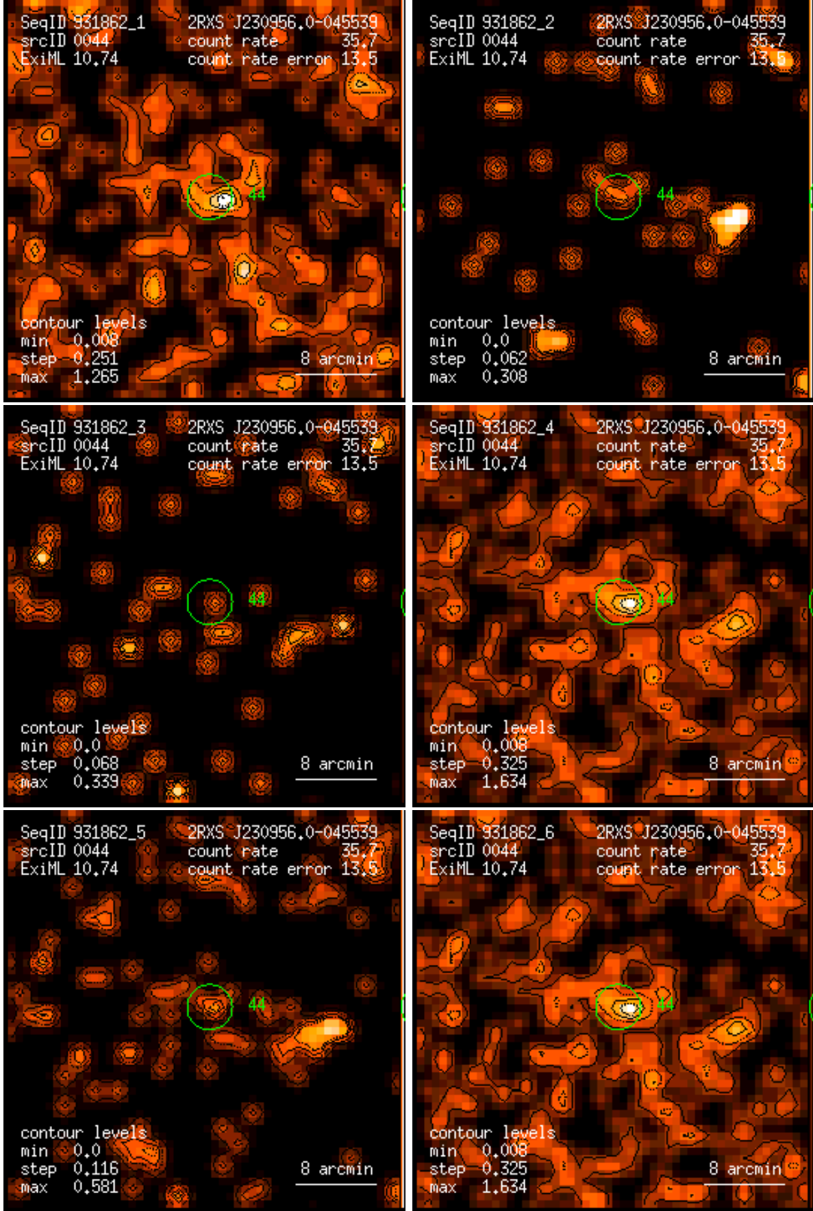
Figure 44: RASS 931862: detection 0044: band rate images, Gaussian filter: (1) PSPC channels 11 – 41, (2) 52 – 90, (3) 91 – 201, (4) 11 – 235, (5) 52 – 201, (6) 11 – 201. Broad band rates in counts/ks. Band rate contour levels in counts/ks/arcmin 2 .
