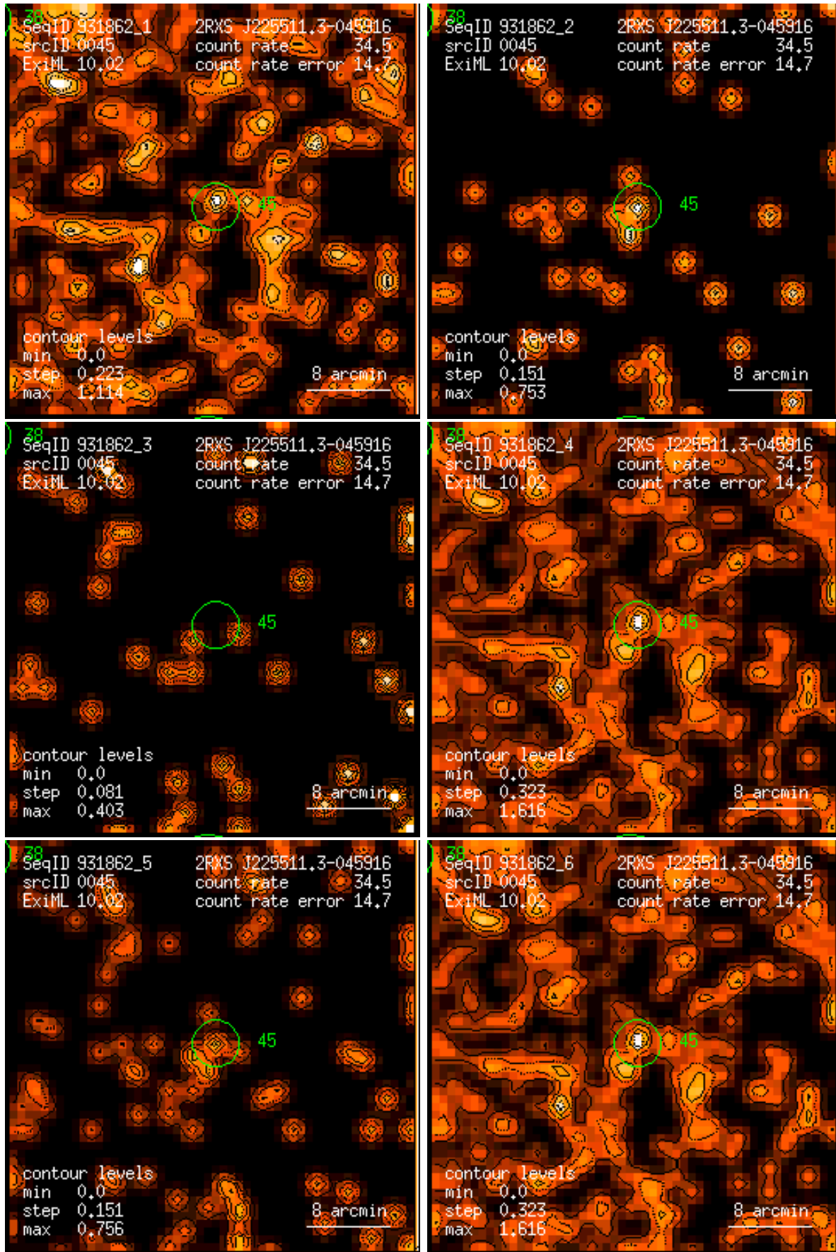
Figure 45: RASS 931862: detection 0045: band rate images, Gaussian filter: (1) PSPC channels 11 – 41, (2) 52 – 90, (3) 91 – 201, (4) 11 – 235, (5) 52 – 201, (6) 11 – 201. Broad band rates in counts/ks. Band rate contour levels in counts/ks/arcmin 2 .
