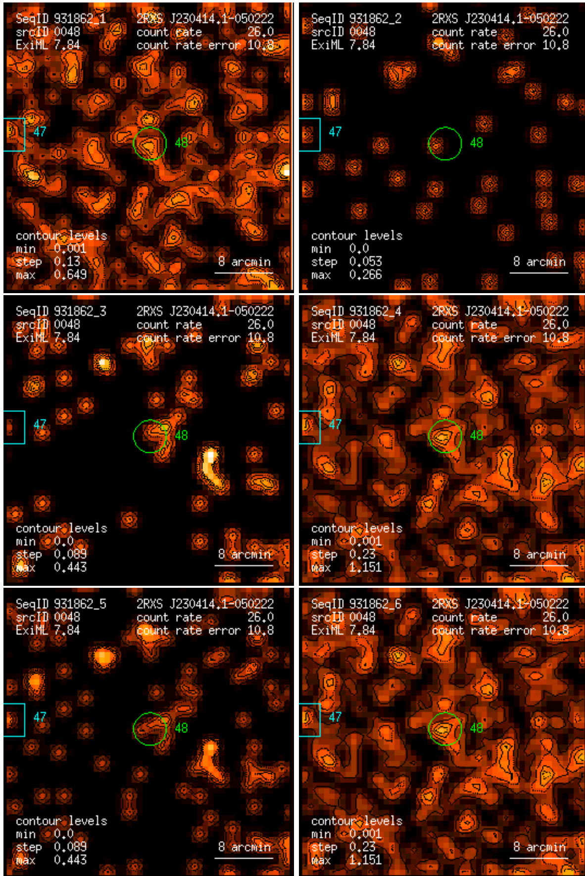
Figure 48: RASS 931862: detection 0048: band rate images, Gaussian filter: (1) PSPC channels 11 – 41, (2) 52 – 90, (3) 91 – 201, (4) 11 – 235, (5) 52 – 201, (6) 11 – 201. Broad band rates in counts/ks. Band rate contour levels in counts/ks/arcmin 2 .
