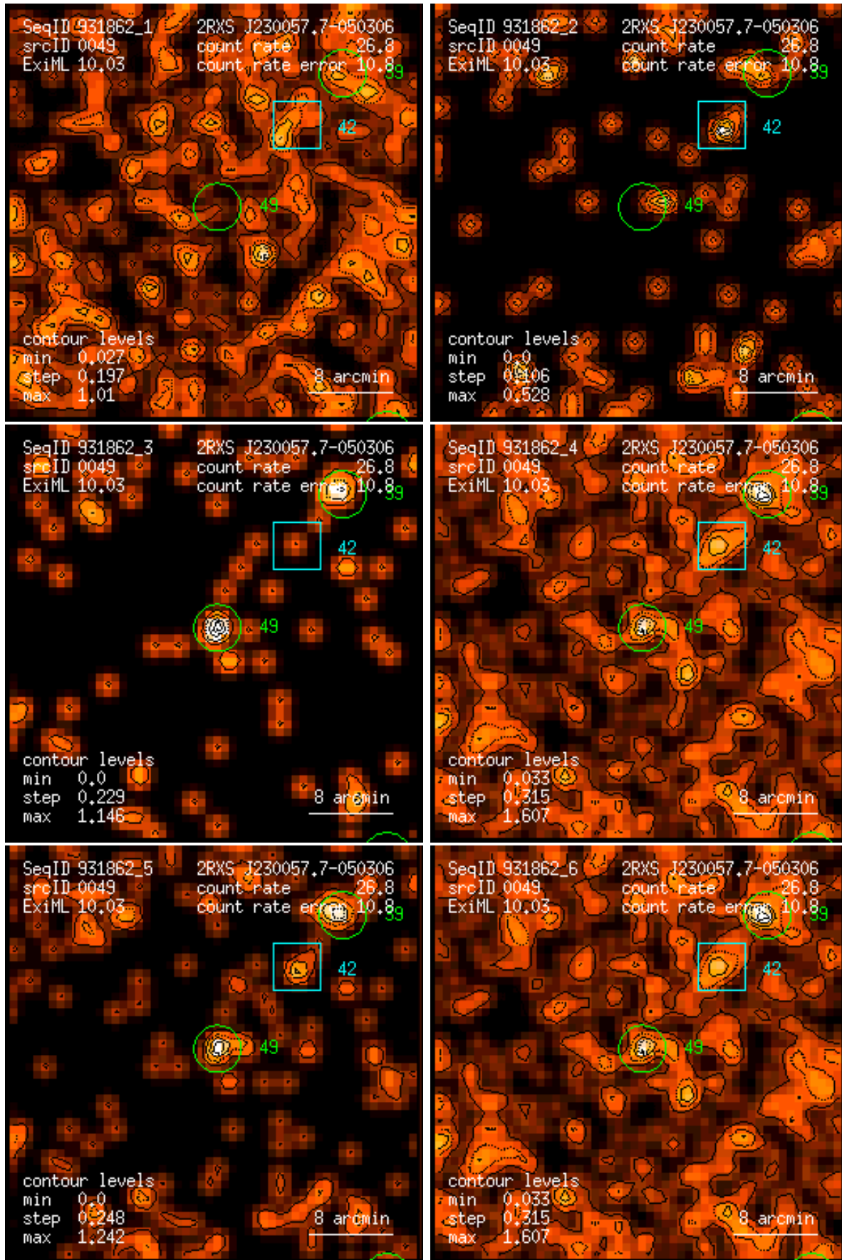
Figure 49: RASS 931862: detection 0049: band rate images, Gaussian filter: (1) PSPC channels 11 – 41, (2) 52 – 90, (3) 91 – 201, (4) 11 – 235, (5) 52 – 201, (6) 11 – 201. Broad band rates in counts/ks. Band rate contour levels in counts/ks/arcmin 2 .
