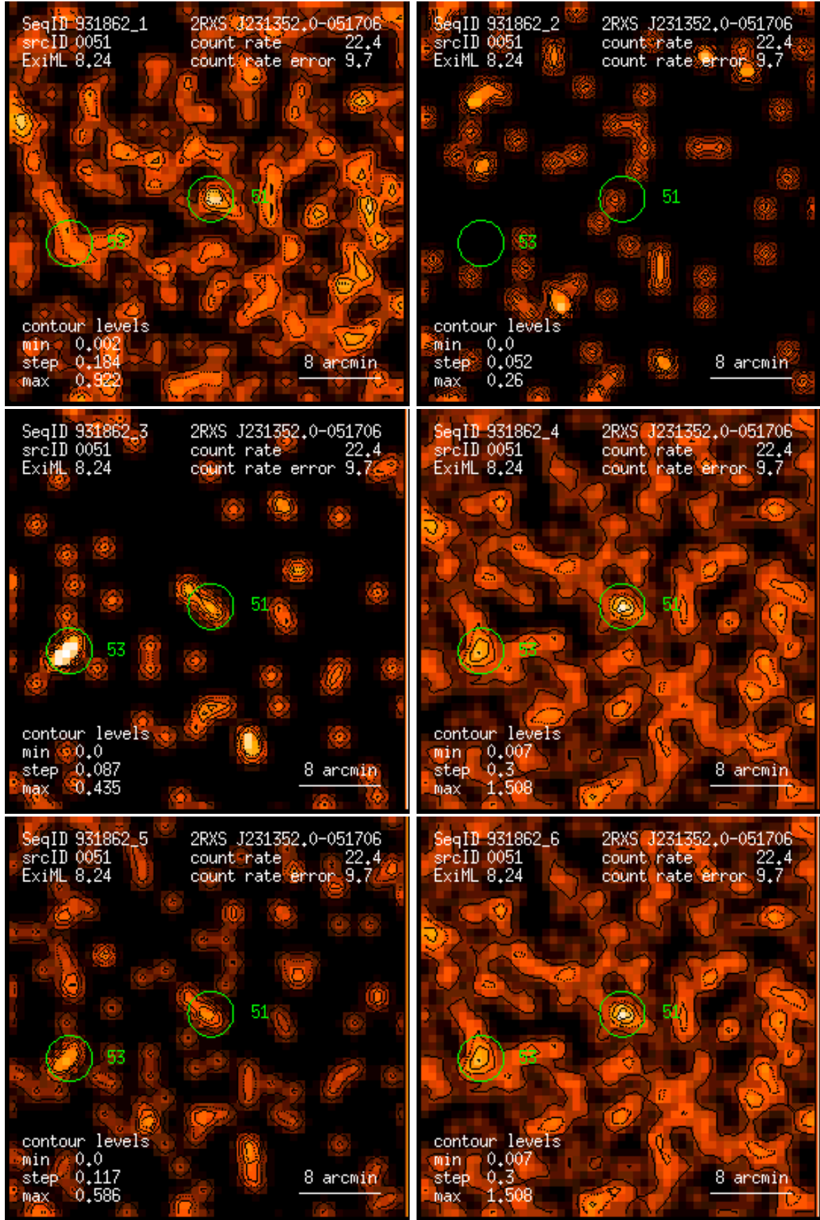
Figure 51: RASS 931862: detection 0051: band rate images, Gaussian filter: (1) PSPC channels 11 – 41, (2) 52 – 90, (3) 91 – 201, (4) 11 – 235, (5) 52 – 201, (6) 11 – 201. Broad band rates in counts/ks. Band rate contour levels in counts/ks/arcmin 2 .
