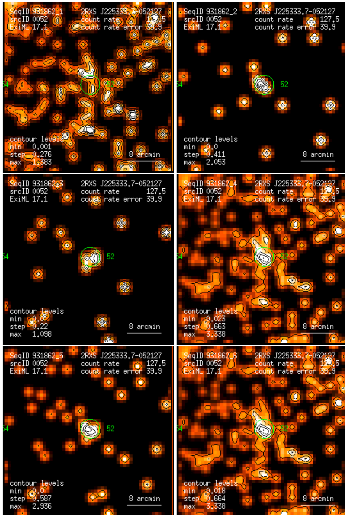
Figure 52: RASS 931862: detection 0052: band rate images, Gaussian filter: (1) PSPC channels 11 – 41, (2) 52 – 90, (3) 91 – 201, (4) 11 – 235, (5) 52 – 201, (6) 11 – 201. Broad band rates in counts/ks. Band rate contour levels in counts/ks/arcmin 2 .
