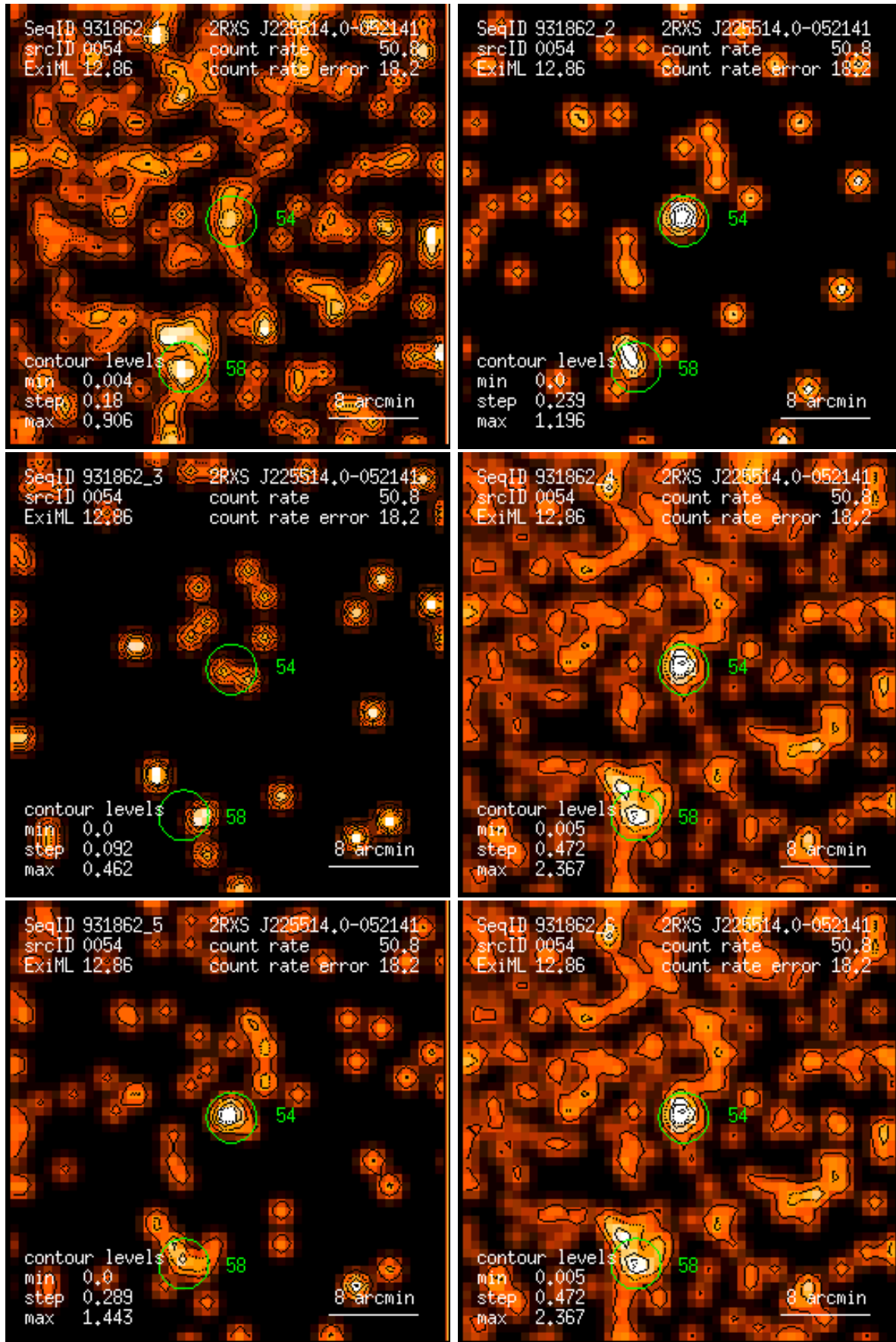
Figure 54: RASS 931862: detection 0054: band rate images, Gaussian filter: (1) PSPC channels 11 – 41, (2) 52 – 90, (3) 91 – 201, (4) 11 – 235, (5) 52 – 201, (6) 11 – 201. Broad band rates in counts/ks. Band rate contour levels in counts/ks/arcmin 2 .
