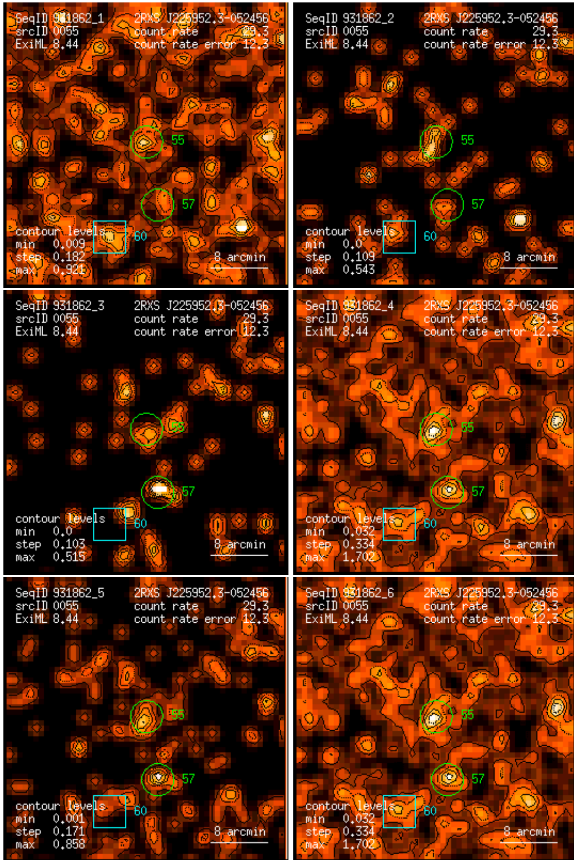
Figure 55: RASS 931862: detection 0055: band rate images, Gaussian filter: (1) PSPC channels 11 – 41, (2) 52 – 90, (3) 91 – 201, (4) 11 – 235, (5) 52 – 201, (6) 11 – 201. Broad band rates in counts/ks. Band rate contour levels in counts/ks/arcmin 2 .
