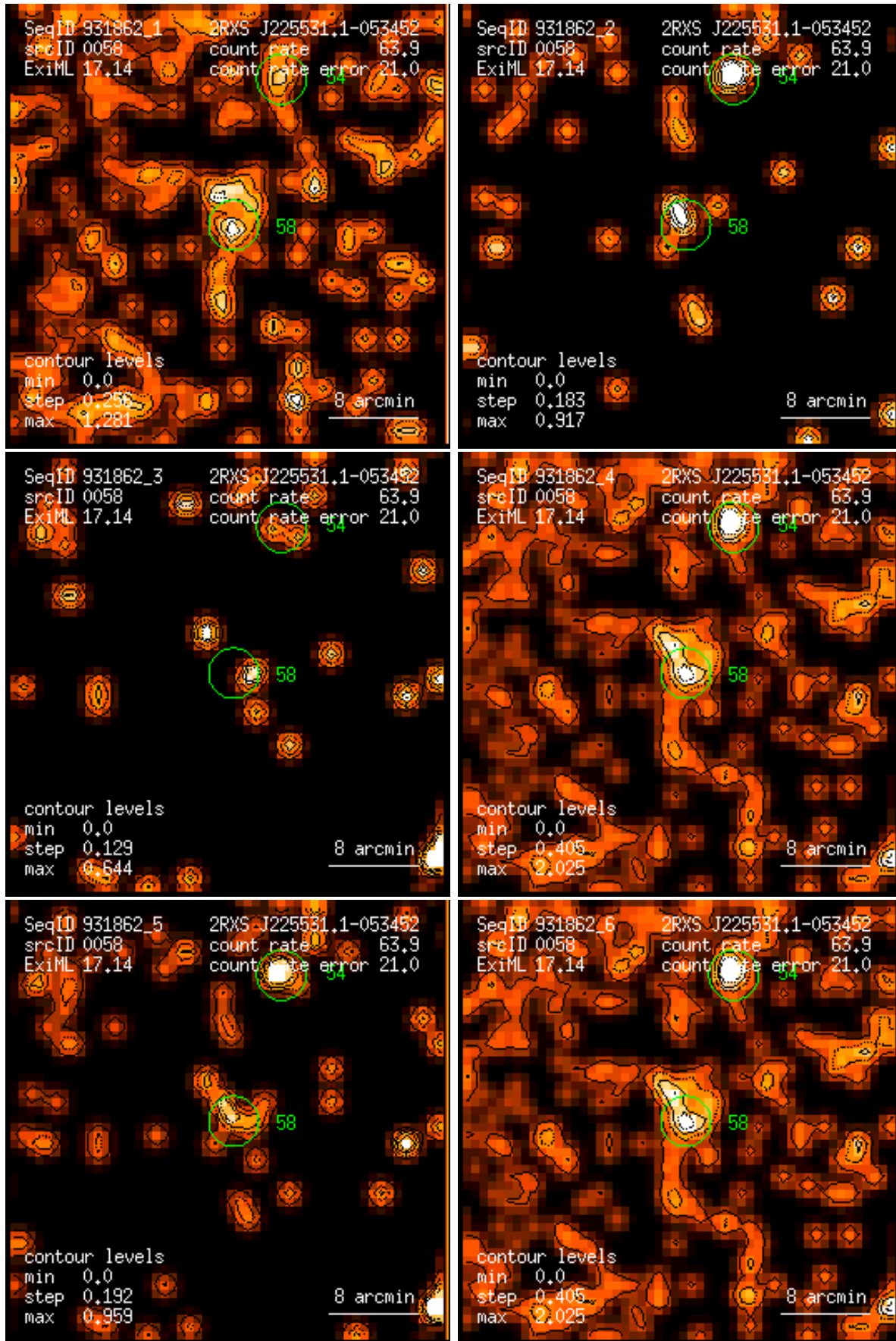
Figure 58: RASS 931862: detection 0058: band rate images, Gaussian filter: (1) PSPC channels 11 – 41, (2) 52 – 90, (3) 91 – 201, (4) 11 – 235, (5) 52 – 201, (6) 11 – 201. Broad band rates in counts/ks. Band rate contour levels in counts/ks/arcmin 2 .
