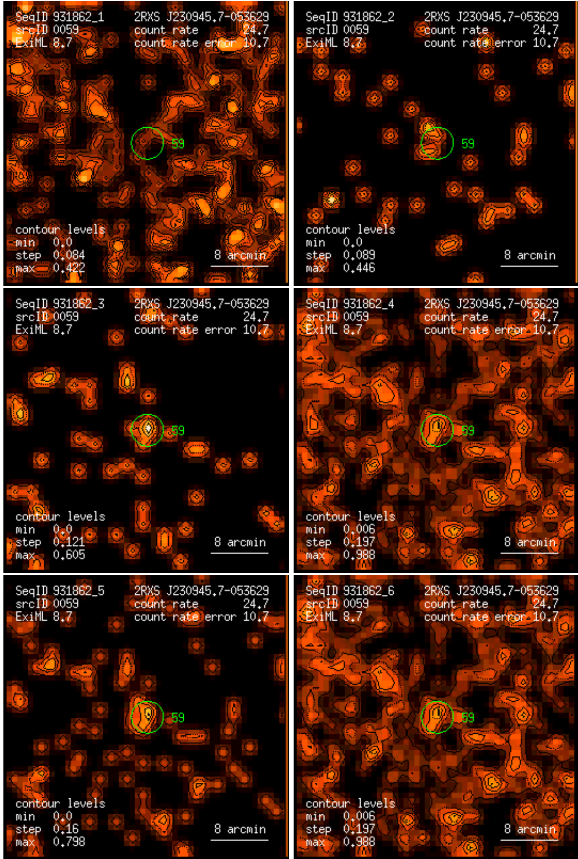
Figure 59: RASS 931862: detection 0059: band rate images, Gaussian filter: (1) PSPC channels 11 – 41, (2) 52 – 90, (3) 91 – 201, (4) 11 – 235, (5) 52 – 201, (6) 11 – 201. Broad band rates in counts/ks. Band rate contour levels in counts/ks/arcmin 2 .
