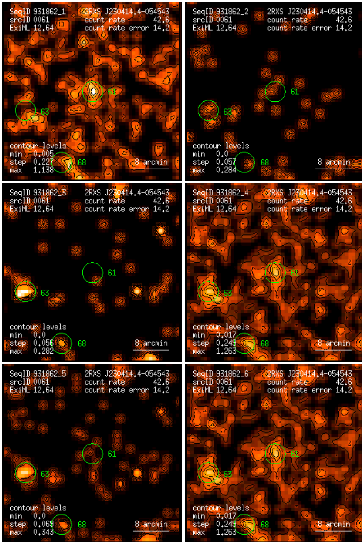
Figure 61: RASS 931862: detection 0061: band rate images, Gaussian filter: (1) PSPC channels 11 – 41, (2) 52 – 90, (3) 91 – 201, (4) 11 – 235, (5) 52 – 201, (6) 11 – 201. Broad band rates in counts/ks. Band rate contour levels in counts/ks/arcmin 2 .
