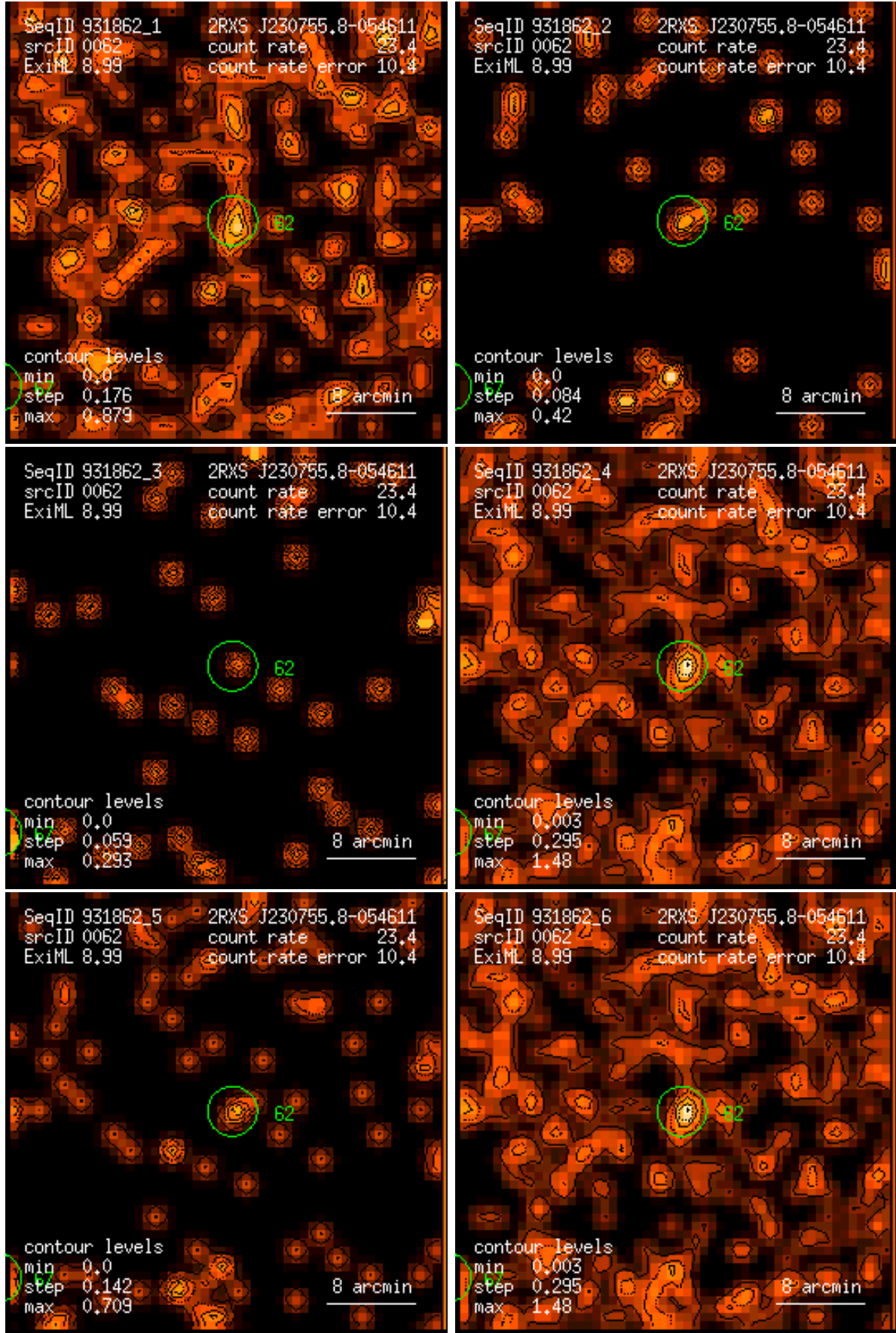
Figure 62: RASS 931862: detection 0062: band rate images, Gaussian filter: (1) PSPC channels 11 – 41, (2) 52 – 90, (3) 91 – 201, (4) 11 – 235, (5) 52 – 201, (6) 11 – 201. Broad band rates in counts/ks. Band rate contour levels in counts/ks/arcmin 2 .
