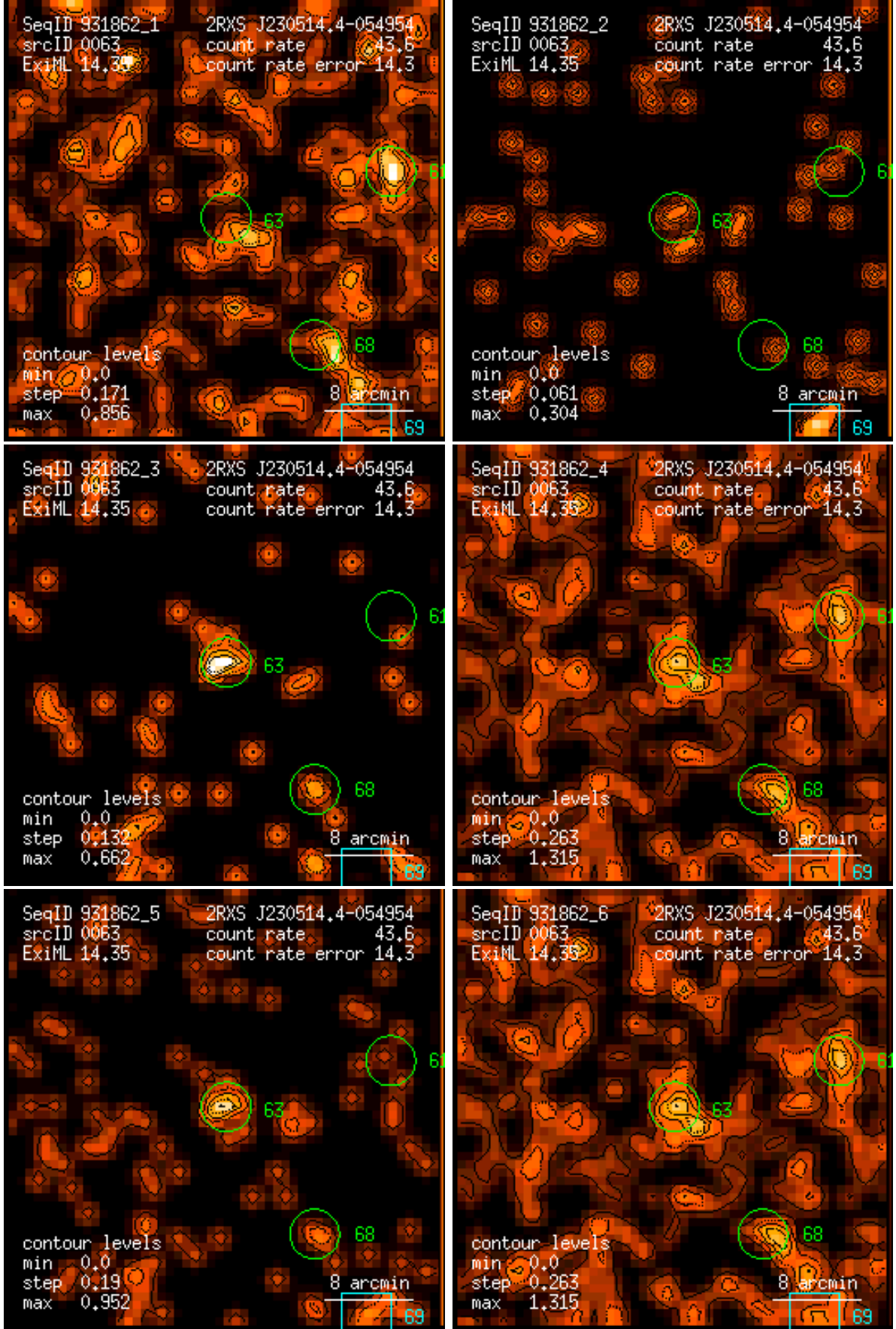
Figure 63: RASS 931862: detection 0063: band rate images, Gaussian filter: (1) PSPC channels 11 – 41, (2) 52 – 90, (3) 91 – 201, (4) 11 – 235, (5) 52 – 201, (6) 11 – 201. Broad band rates in counts/ks. Band rate contour levels in counts/ks/arcmin 2 .
