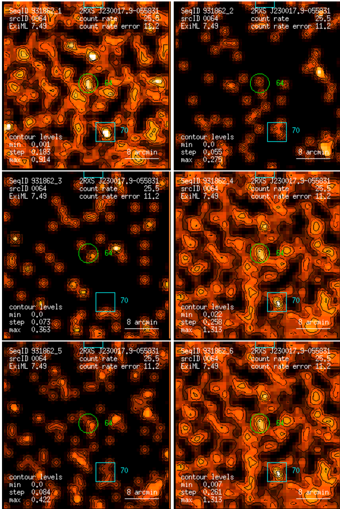
Figure 64: RASS 931862: detection 0064: band rate images, Gaussian filter: (1) PSPC channels 11 – 41, (2) 52 – 90, (3) 91 – 201, (4) 11 – 235, (5) 52 – 201, (6) 11 – 201. Broad band rates in counts/ks. Band rate contour levels in counts/ks/arcmin 2 .
