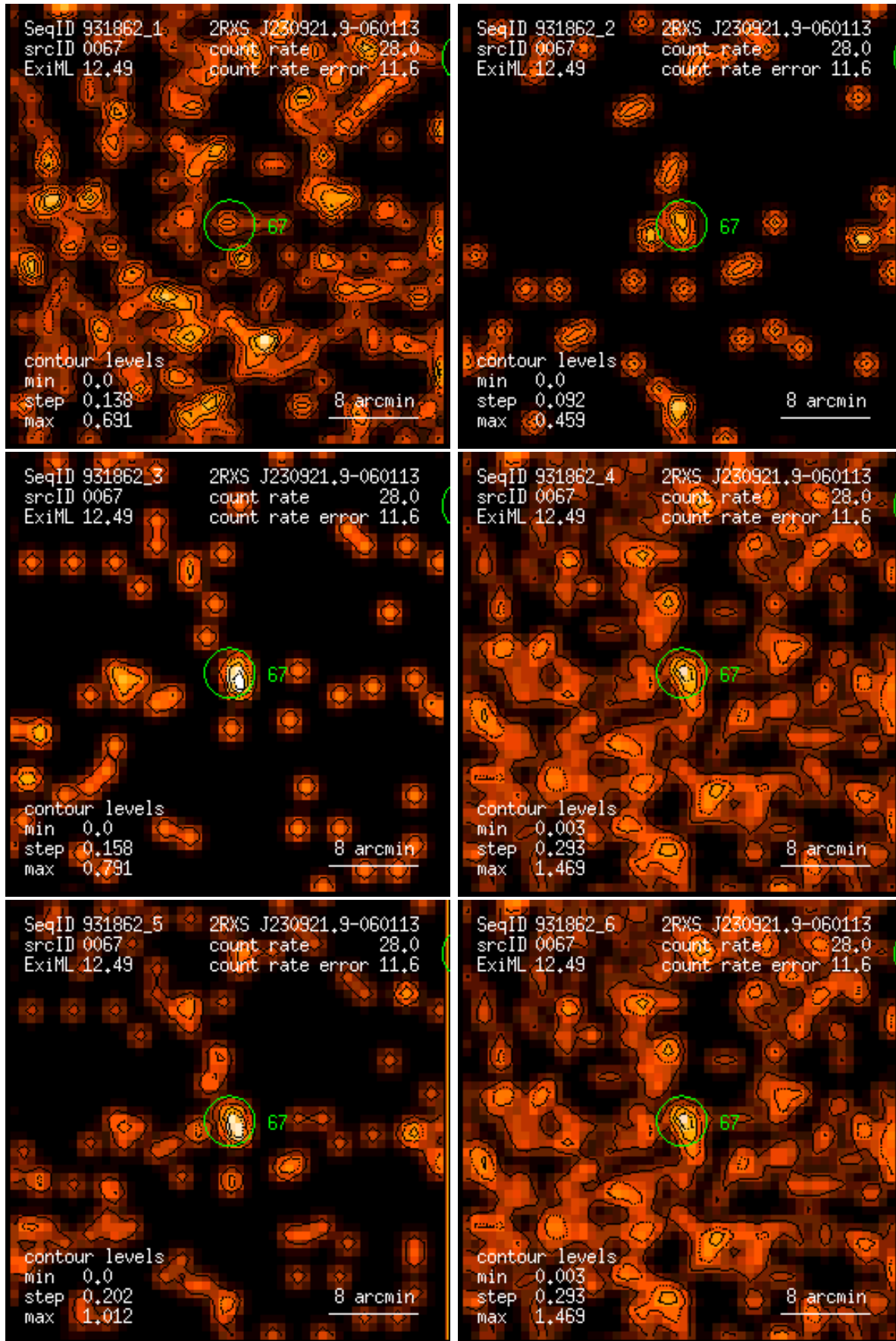
Figure 67: RASS 931862: detection 0067: band rate images, Gaussian filter: (1) PSPC channels 11 – 41, (2) 52 – 90, (3) 91 – 201, (4) 11 – 235, (5) 52 – 201, (6) 11 – 201. Broad band rates in counts/ks. Band rate contour levels in counts/ks/arcmin 2 .
