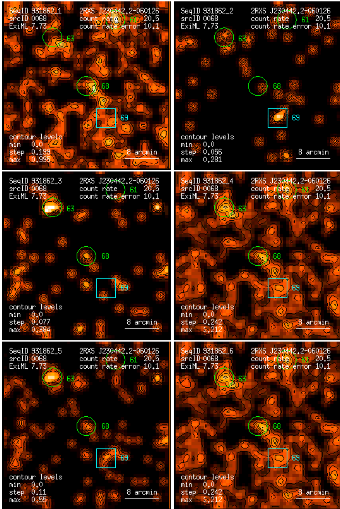
Figure 68: RASS 931862: detection 0068: band rate images, Gaussian filter: (1) PSPC channels 11 – 41, (2) 52 – 90, (3) 91 – 201, (4) 11 – 235, (5) 52 – 201, (6) 11 – 201. Broad band rates in counts/ks. Band rate contour levels in counts/ks/arcmin 2 .
