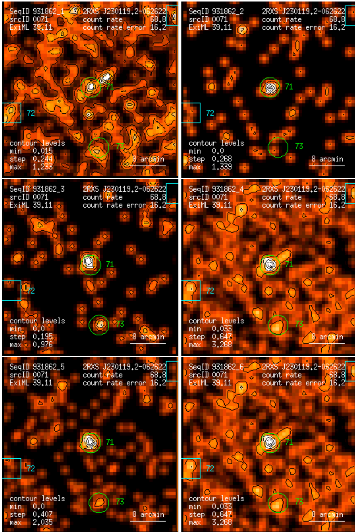
Figure 71: RASS 931862: detection 0071: band rate images, Gaussian filter: (1) PSPC channels 11 – 41, (2) 52 – 90, (3) 91 – 201, (4) 11 – 235, (5) 52 – 201, (6) 11 – 201. Broad band rates in counts/ks. Band rate contour levels in counts/ks/arcmin 2 .
