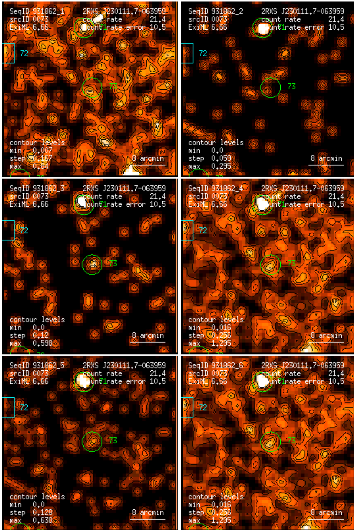
Figure 73: RASS 931862: detection 0073: band rate images, Gaussian filter: (1) PSPC channels 11 – 41, (2) 52 – 90, (3) 91 – 201, (4) 11 – 235, (5) 52 – 201, (6) 11 – 201. Broad band rates in counts/ks. Band rate contour levels in counts/ks/arcmin 2 .
