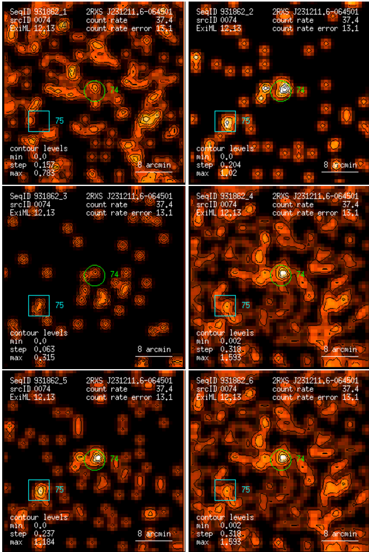
Figure 74: RASS 931862: detection 0074: band rate images, Gaussian filter: (1) PSPC channels 11 – 41, (2) 52 – 90, (3) 91 – 201, (4) 11 – 235, (5) 52 – 201, (6) 11 – 201. Broad band rates in counts/ks. Band rate contour levels in counts/ks/arcmin 2 .
