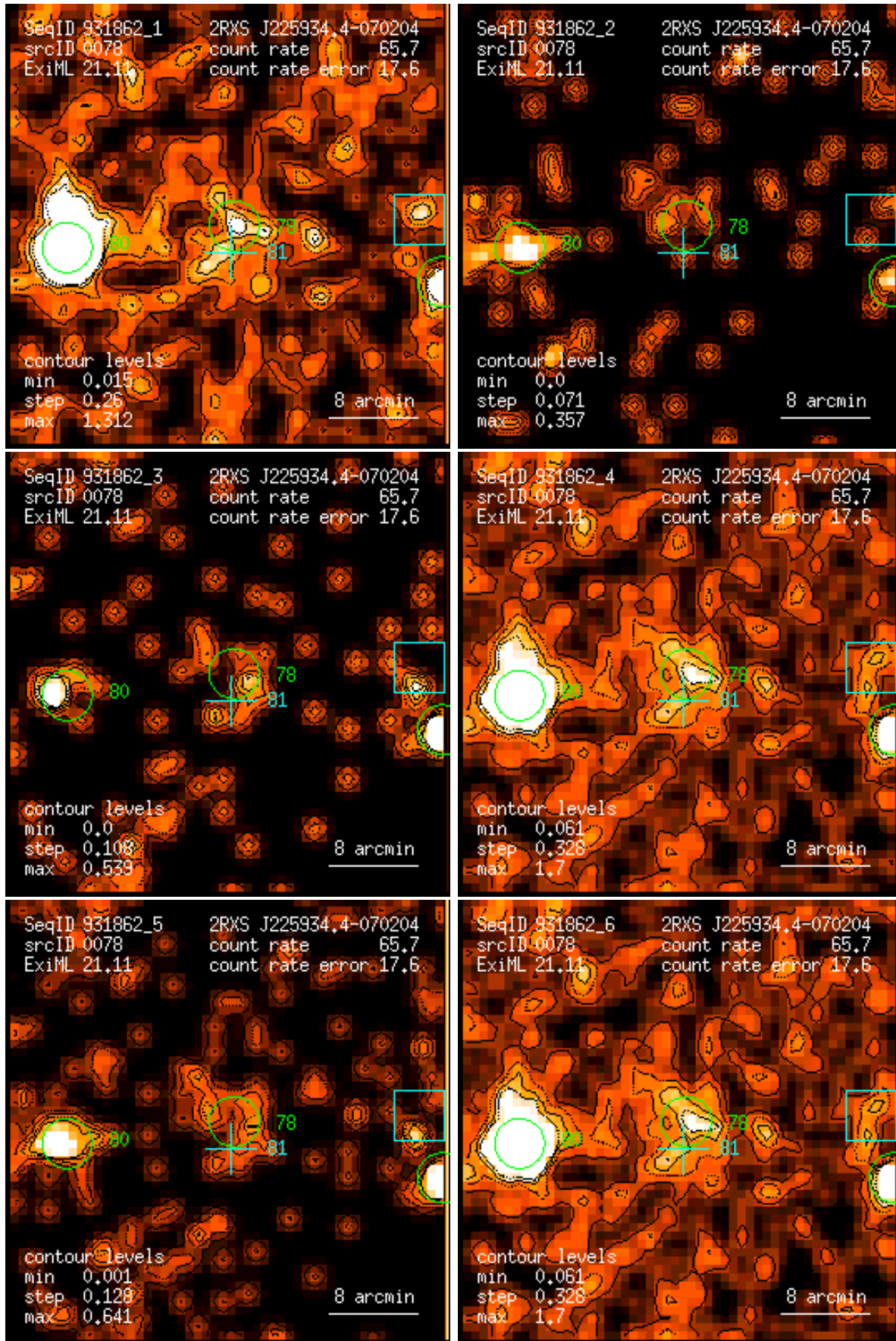
Figure 78: RASS 931862: detection 0078: band rate images, Gaussian filter: (1) PSPC channels 11 – 41, (2) 52 – 90, (3) 91 – 201, (4) 11 – 235, (5) 52 – 201, (6) 11 – 201. Broad band rates in counts/ks. Band rate contour levels in counts/ks/arcmin 2 .
