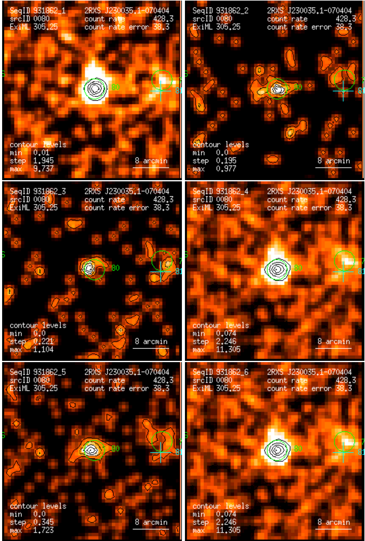
Figure 80: RASS 931862: detection 0080: band rate images, Gaussian filter: (1) PSPC channels 11 – 41, (2) 52 – 90, (3) 91 – 201, (4) 11 – 235, (5) 52 – 201, (6) 11 – 201. Broad band rates in counts/ks. Band rate contour levels in counts/ks/arcmin 2 .
