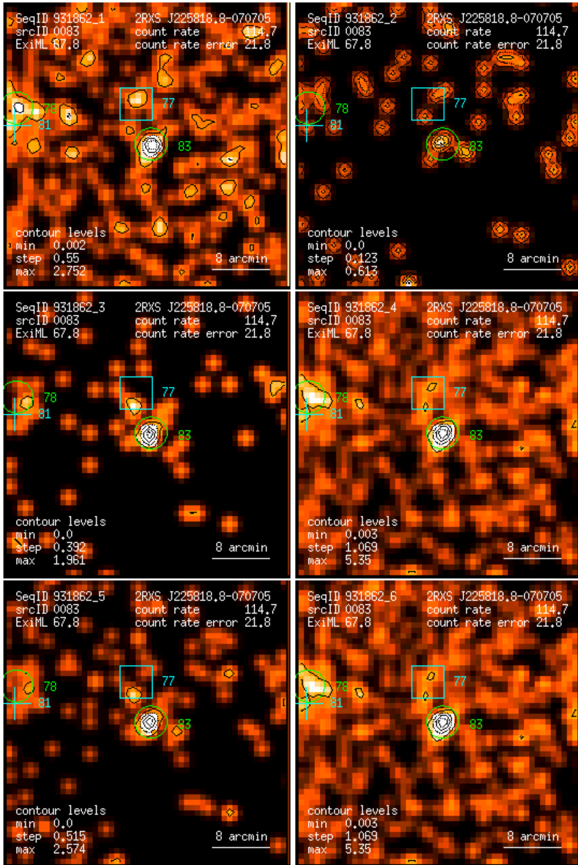
Figure 83: RASS 931862: detection 0083: band rate images, Gaussian filter: (1) PSPC channels 11 – 41, (2) 52 – 90, (3) 91 – 201, (4) 11 – 235, (5) 52 – 201, (6) 11 – 201. Broad band rates in counts/ks. Band rate contour levels in counts/ks/arcmin 2 .
