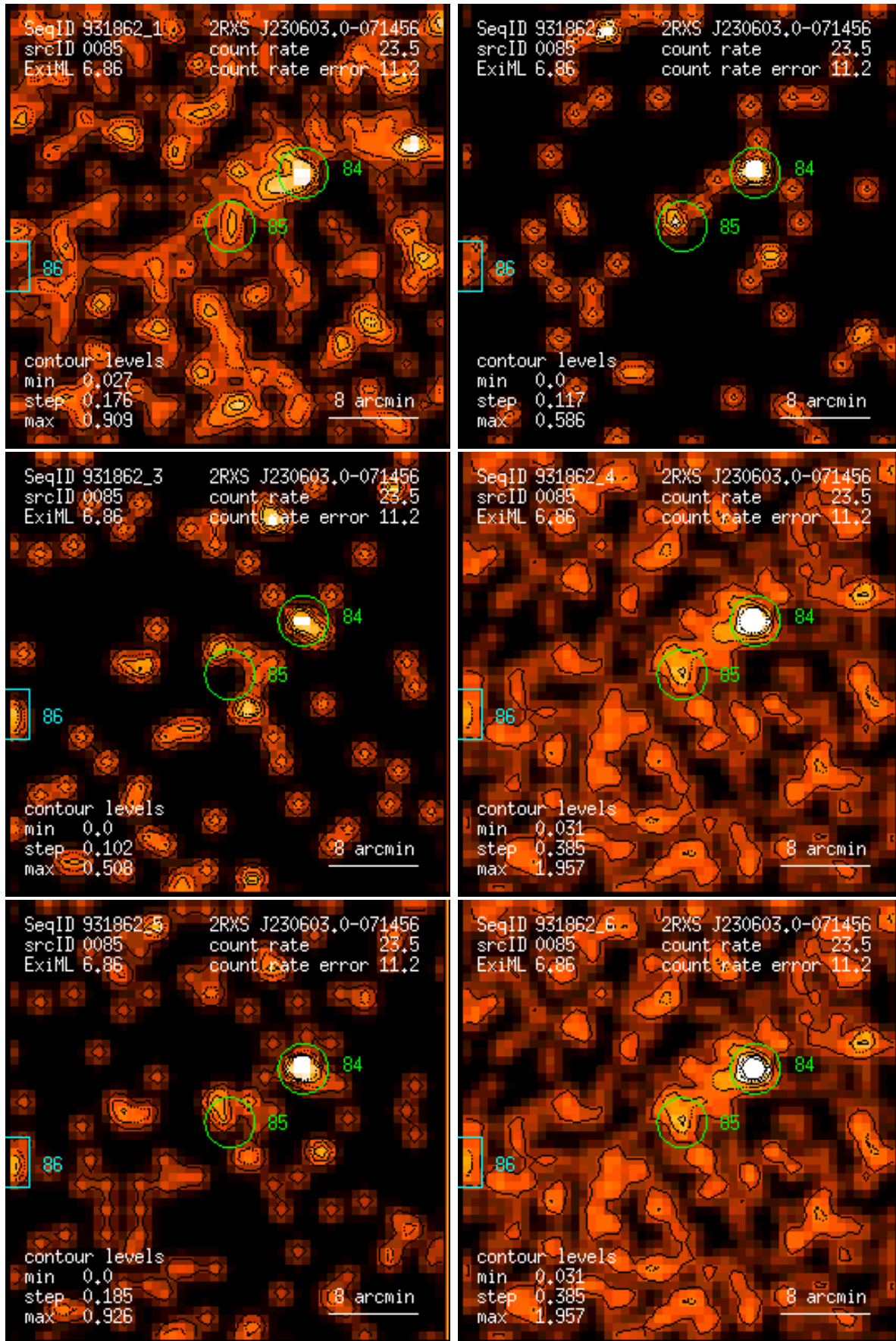
Figure 85: RASS 931862: detection 0085: band rate images, Gaussian filter: (1) PSPC channels 11 – 41, (2) 52 – 90, (3) 91 – 201, (4) 11 – 235, (5) 52 – 201, (6) 11 – 201. Broad band rates in counts/ks. Band rate contour levels in counts/ks/arcmin 2 .
