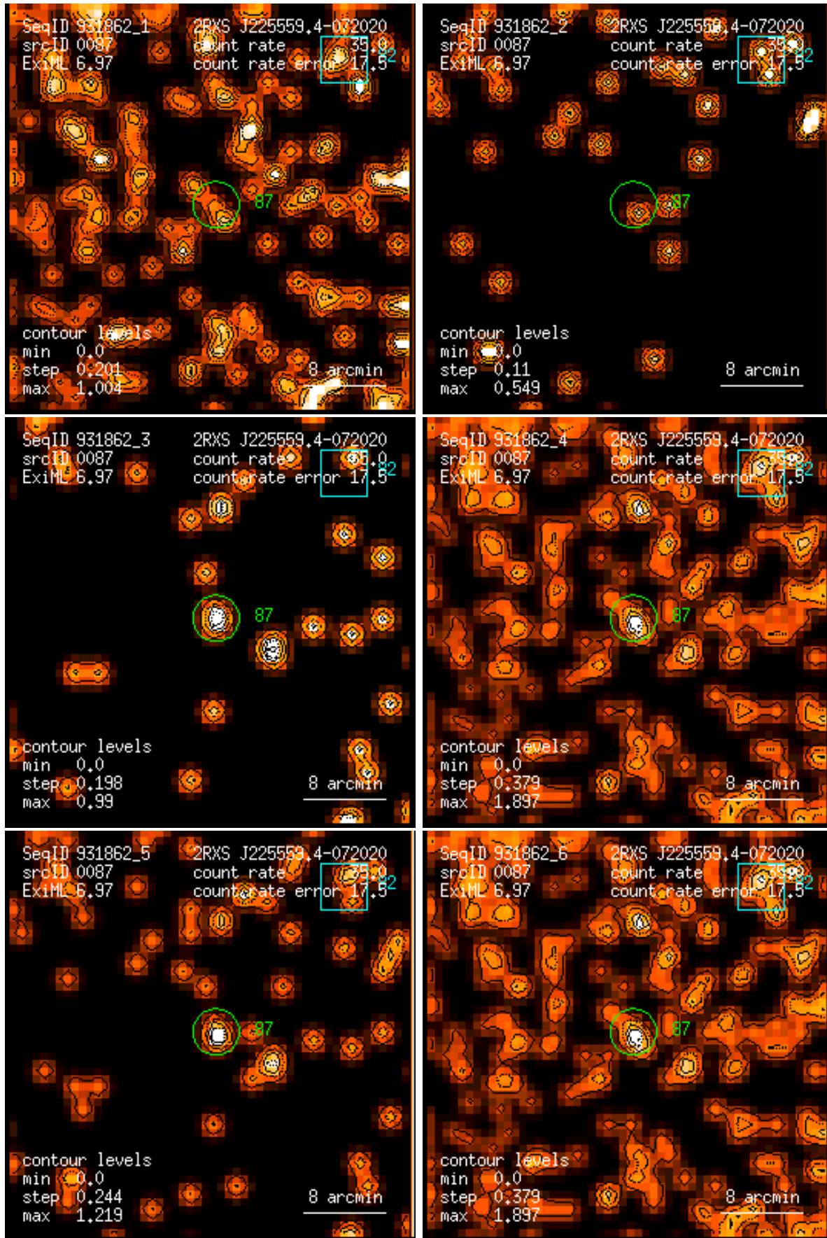
Figure 87: RASS 931862: detection 0087: band rate images, Gaussian filter: (1) PSPC channels 11 – 41, (2) 52 – 90, (3) 91 – 201, (4) 11 – 235, (5) 52 – 201, (6) 11 – 201. Broad band rates in counts/ks. Band rate contour levels in counts/ks/arcmin 2 .
