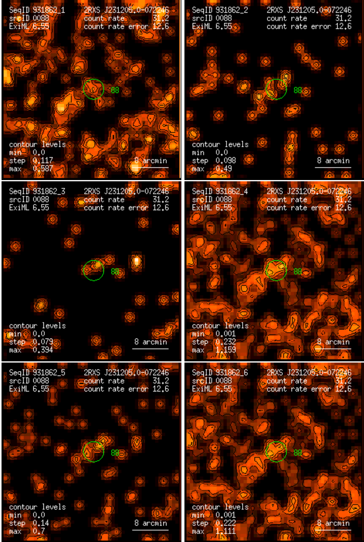
Figure 88: RASS 931862: detection 0088: band rate images, Gaussian filter: (1) PSPC channels 11 – 41, (2) 52 – 90, (3) 91 – 201, (4) 11 – 235, (5) 52 – 201, (6) 11 – 201. Broad band rates in counts/ks. Band rate contour levels in counts/ks/arcmin 2 .
