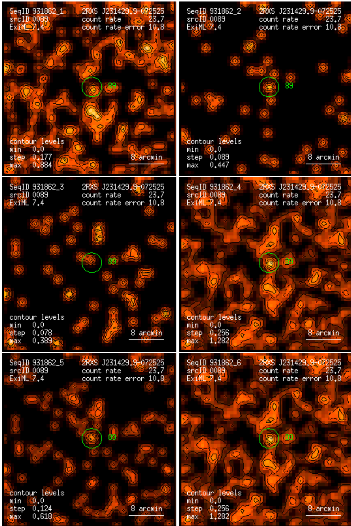
Figure 89: RASS 931862: detection 0089: band rate images, Gaussian filter: (1) PSPC channels 11 – 41, (2) 52 – 90, (3) 91 – 201, (4) 11 – 235, (5) 52 – 201, (6) 11 – 201. Broad band rates in counts/ks. Band rate contour levels in counts/ks/arcmin 2 .
