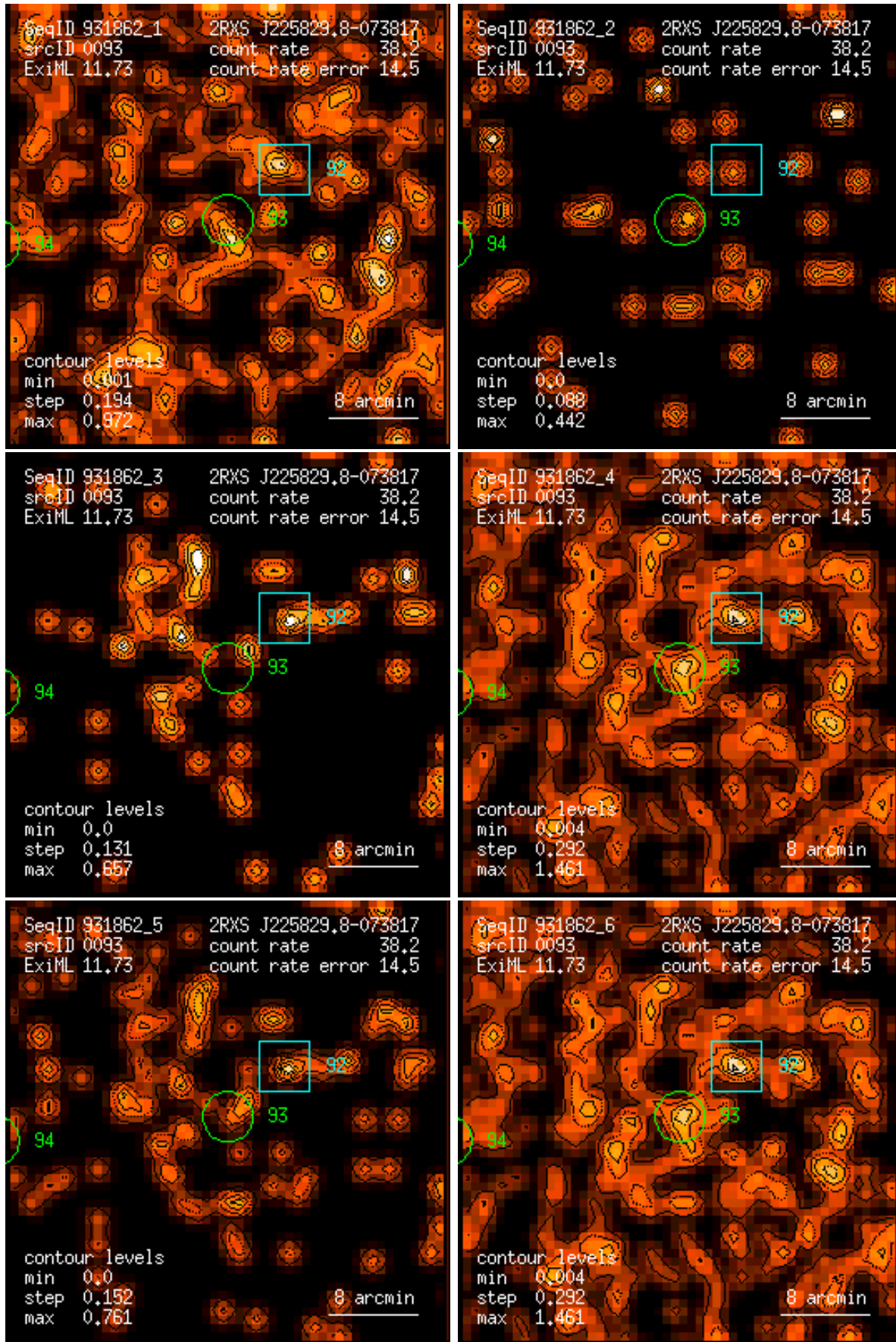
Figure 93: RASS 931862: detection 0093: band rate images, Gaussian filter: (1) PSPC channels 11 – 41, (2) 52 – 90, (3) 91 – 201, (4) 11 – 235, (5) 52 – 201, (6) 11 – 201. Broad band rates in counts/ks. Band rate contour levels in counts/ks/arcmin 2 .
