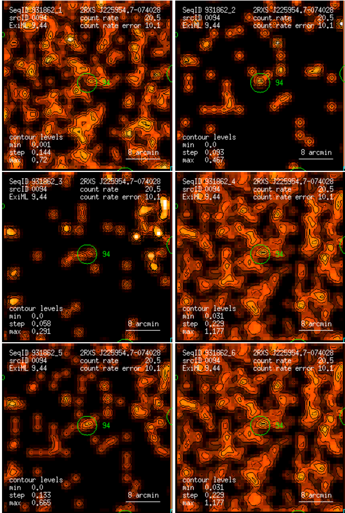
Figure 94: RASS 931862: detection 0094: band rate images, Gaussian filter: (1) PSPC channels 11 – 41, (2) 52 – 90, (3) 91 – 201, (4) 11 – 235, (5) 52 – 201, (6) 11 – 201. Broad band rates in counts/ks. Band rate contour levels in counts/ks/arcmin 2 .
