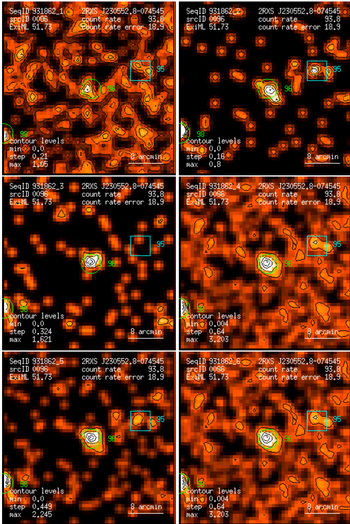
Figure 96: RASS 931862: detection 0096: band rate images, Gaussian filter: (1) PSPC channels 11 – 41, (2) 52 – 90, (3) 91 – 201, (4) 11 – 235, (5) 52 – 201, (6) 11 – 201. Broad band rates in counts/ks. Band rate contour levels in counts/ks/arcmin 2 .
