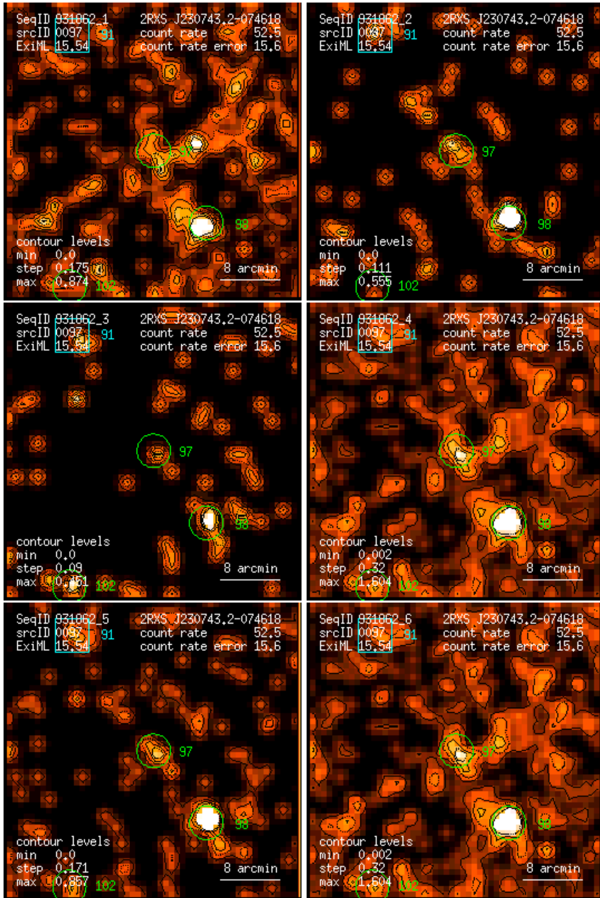
Figure 97: RASS 931862: detection 0097: band rate images, Gaussian filter: (1) PSPC channels 11 – 41, (2) 52 – 90, (3) 91 – 201, (4) 11 – 235, (5) 52 – 201, (6) 11 – 201. Broad band rates in counts/ks. Band rate contour levels in counts/ks/arcmin 2 .
