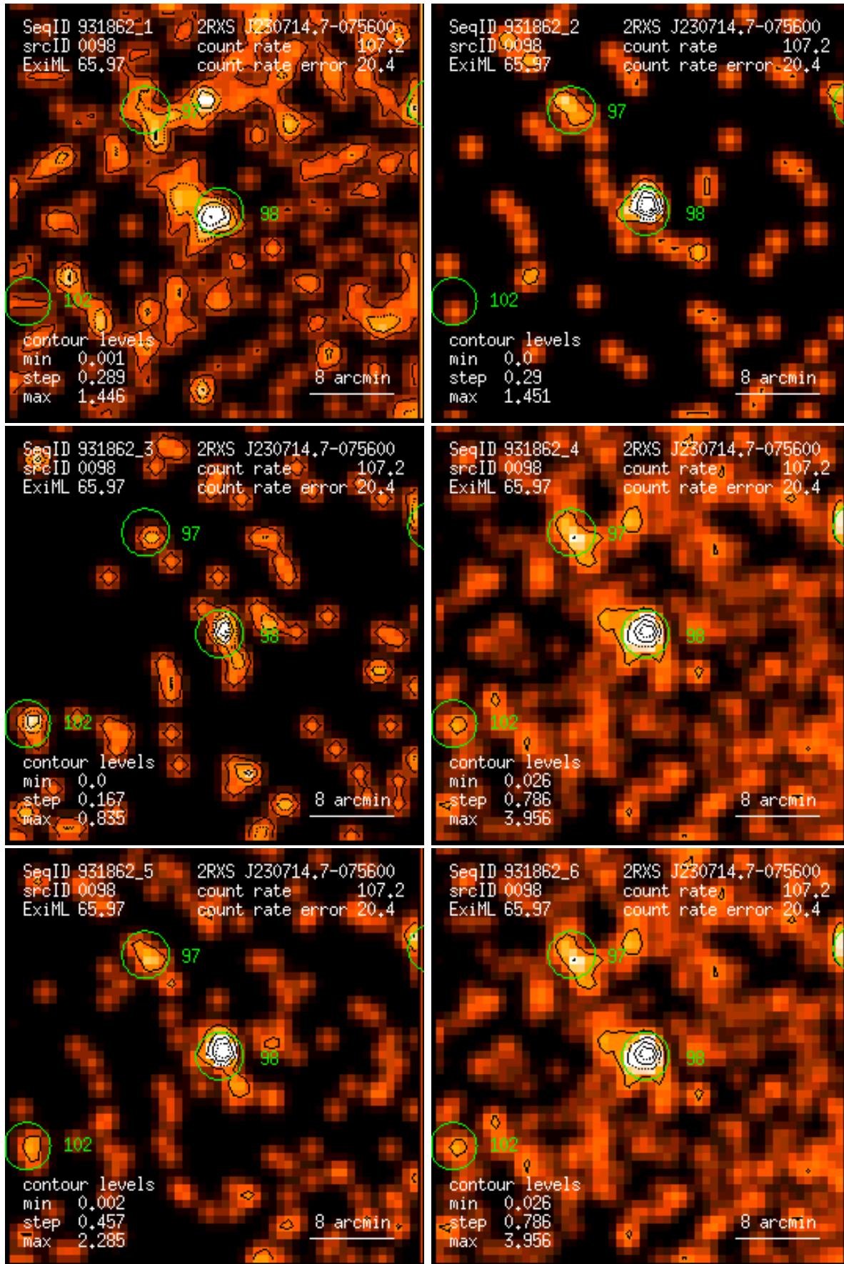
Figure 98: RASS 931862: detection 0098: band rate images, Gaussian filter: (1) PSPC channels 11 – 41, (2) 52 – 90, (3) 91 – 201, (4) 11 – 235, (5) 52 – 201, (6) 11 – 201. Broad band rates in counts/ks. Band rate contour levels in counts/ks/arcmin 2 .
