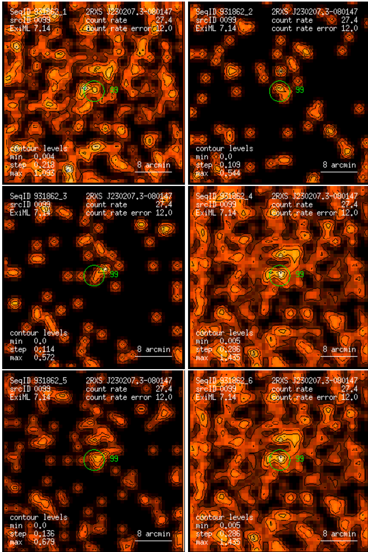
Figure 99: RASS 931862: detection 0099: band rate images, Gaussian filter: (1) PSPC channels 11 – 41, (2) 52 – 90, (3) 91 – 201, (4) 11 – 235, (5) 52 – 201, (6) 11 – 201. Broad band rates in counts/ks. Band rate contour levels in counts/ks/arcmin 2 .
