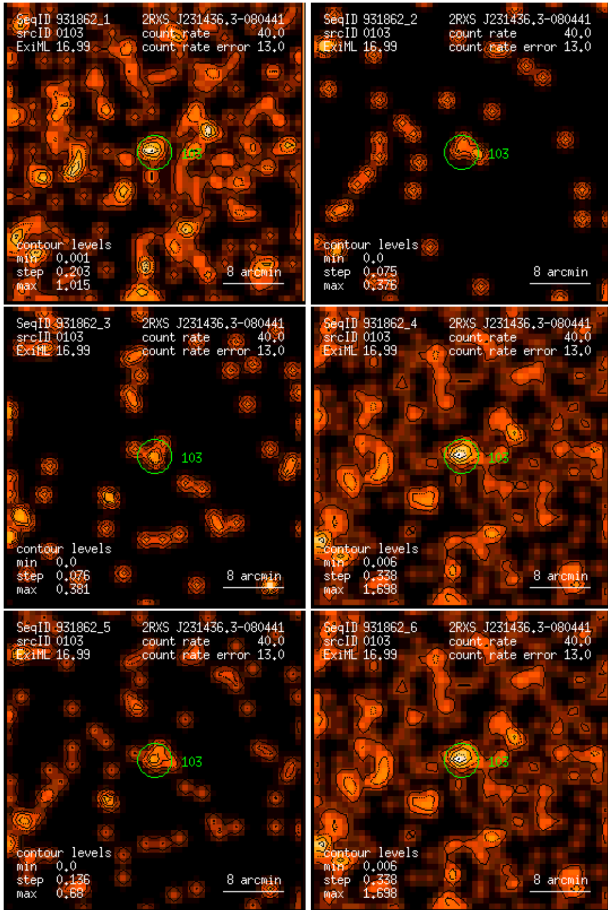
Figure 103: RASS 931862: detection 0103: band rate images, Gaussian filter: (1) PSPC channels 11 – 41, (2) 52 – 90, (3) 91 – 201, (4) 11 – 235, (5) 52 – 201, (6) 11 – 201. Broad band rates in counts/ks. Band rate contour levels in counts/ks/arcmin 2 .
