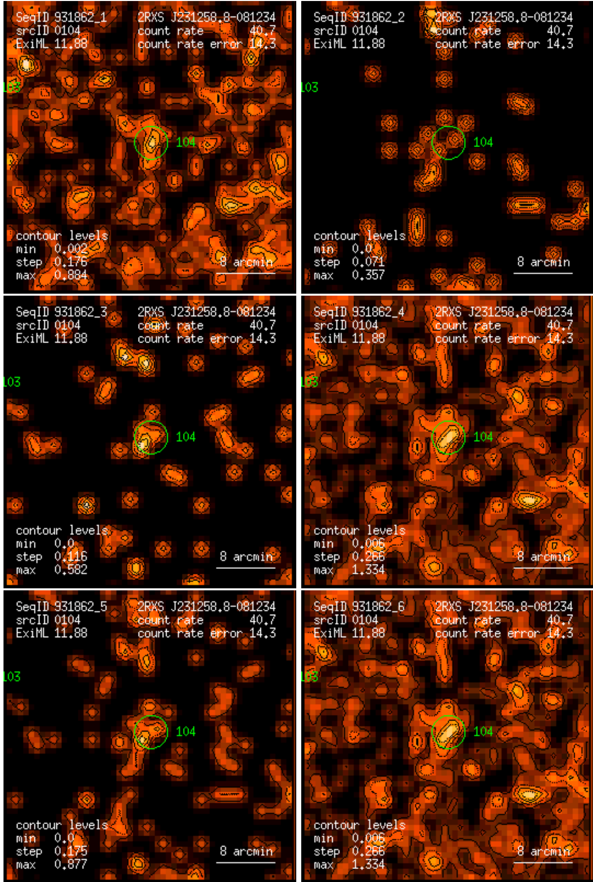
Figure 104: RASS 931862: detection 0104: band rate images, Gaussian filter: (1) PSPC channels 11 – 41, (2) 52 – 90, (3) 91 – 201, (4) 11 – 235, (5) 52 – 201, (6) 11 – 201. Broad band rates in counts/ks. Band rate contour levels in counts/ks/arcmin 2 .
