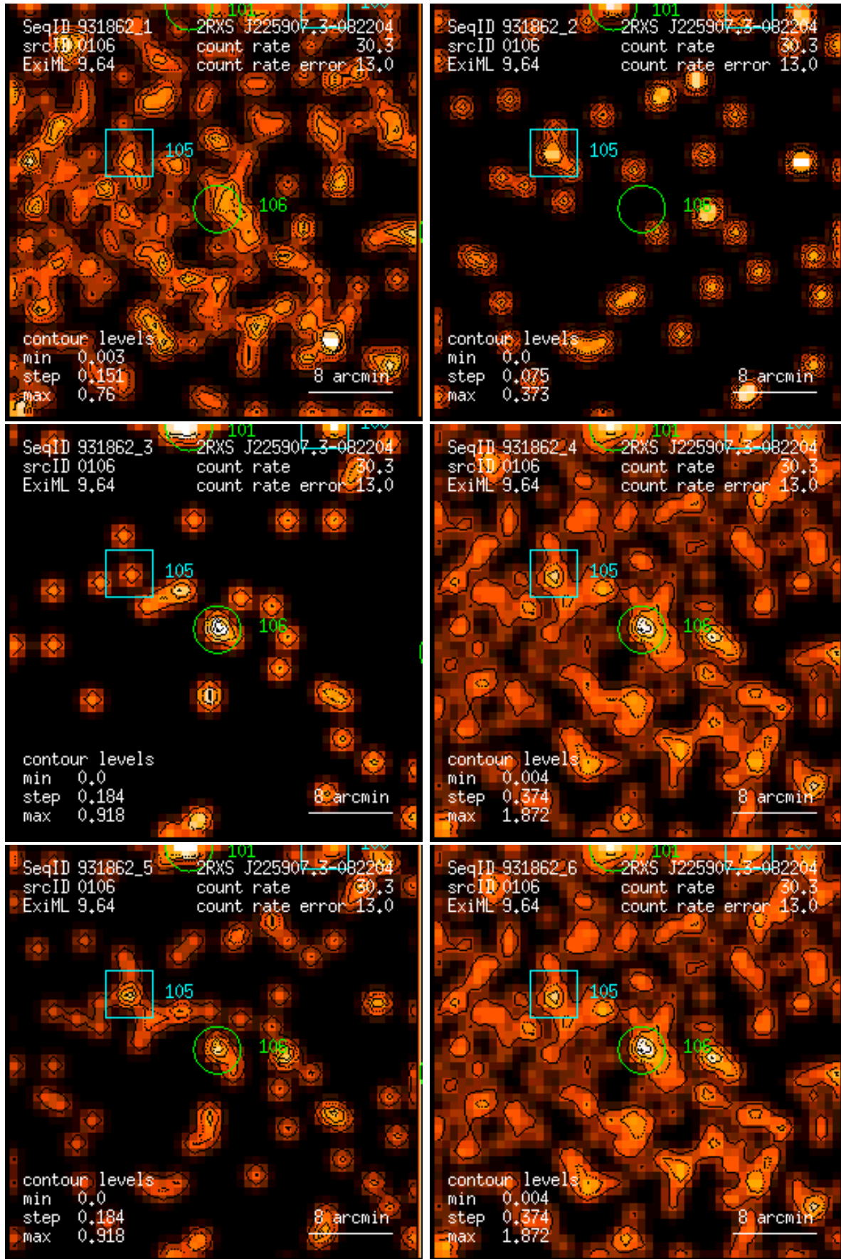
Figure 106: RASS 931862: detection 0106: band rate images, Gaussian filter: (1) PSPC channels 11 – 41, (2) 52 – 90, (3) 91 – 201, (4) 11 – 235, (5) 52 – 201, (6) 11 – 201. Broad band rates in counts/ks. Band rate contour levels in counts/ks/arcmin 2 .
