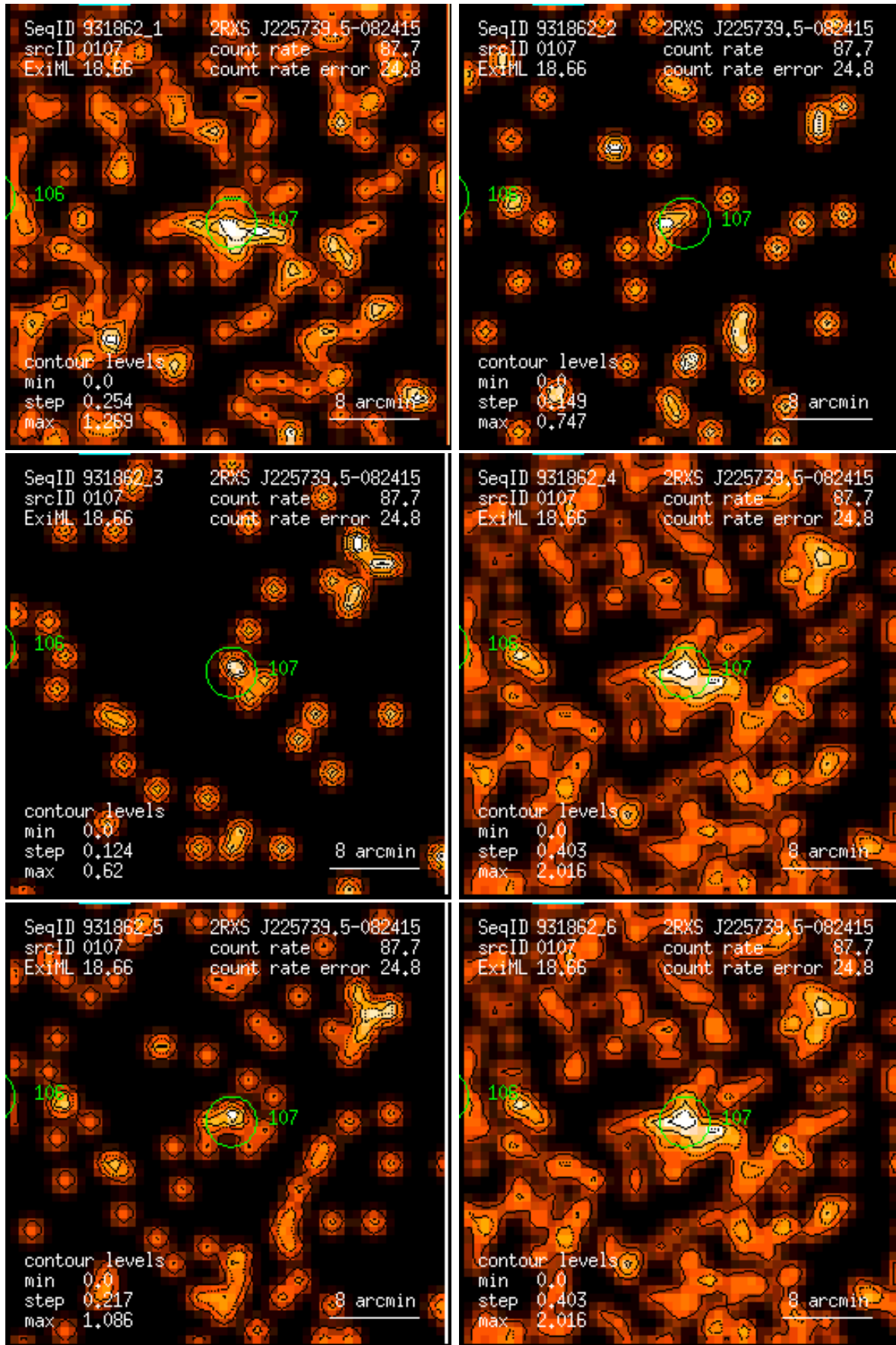
Figure 107: RASS 931862: detection 0107: band rate images, Gaussian filter: (1) PSPC channels 11 – 41, (2) 52 – 90, (3) 91 – 201, (4) 11 – 235, (5) 52 – 201, (6) 11 – 201. Broad band rates in counts/ks. Band rate contour levels in counts/ks/arcmin 2 .
