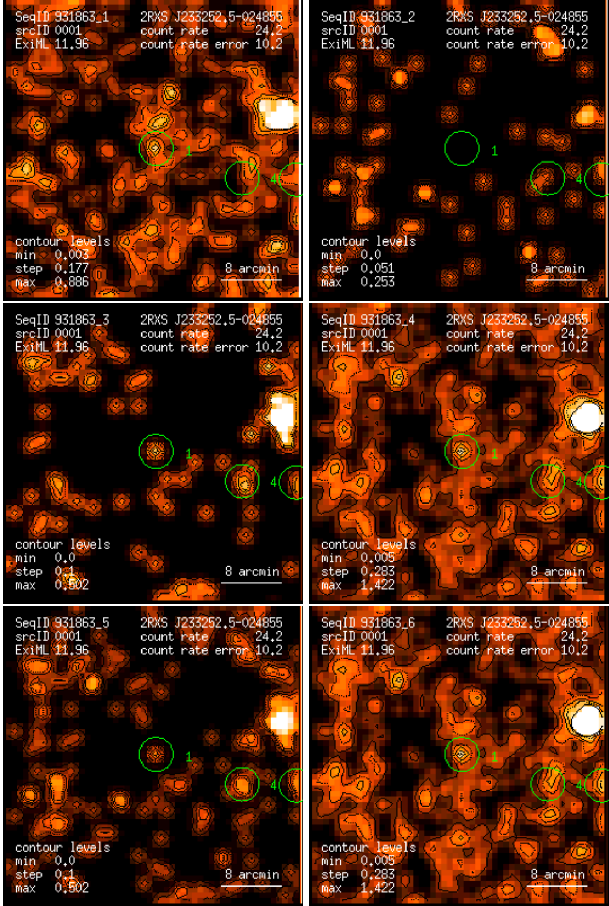
Figure 1: RASS 931863: detection 0001: band rate images, Gaussian filter: (1) PSPC channels 11 – 41, (2) 52 – 90, (3) 91 – 201, (4) 11 – 235, (5) 52 – 201, (6) 11 – 201. Broad band rates in counts/ks. Band rate contour levels in counts/ks/arcmin 2 .
