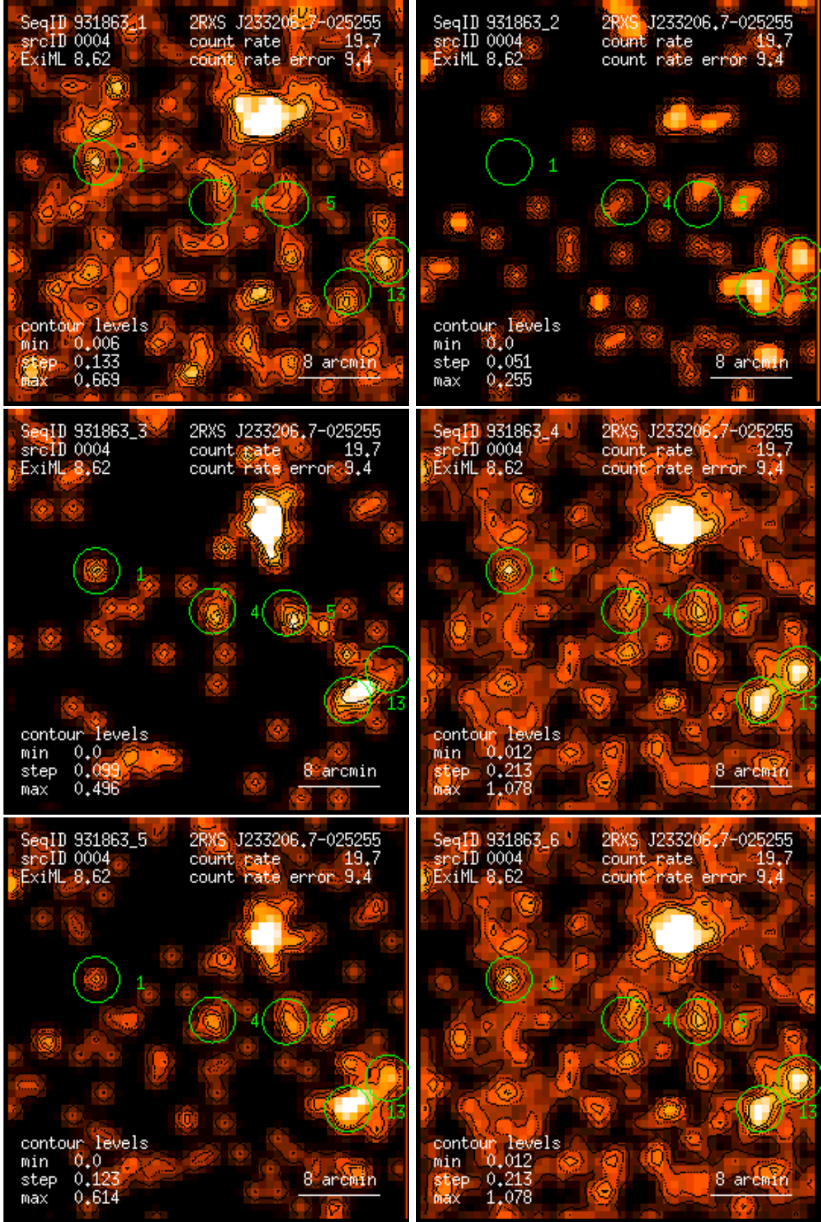
Figure 4: RASS 931863: detection 0004: band rate images, Gaussian filter: (1) PSPC channels 11 – 41, (2) 52 – 90, (3) 91 – 201, (4) 11 – 235, (5) 52 – 201, (6) 11 – 201. Broad band rates in counts/ks. Band rate contour levels in counts/ks/arcmin 2 .
